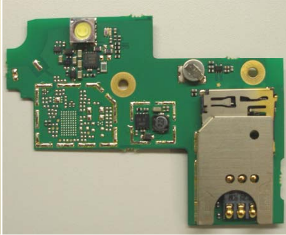
Daughter Board Front (Without Shields and Camera Module)
