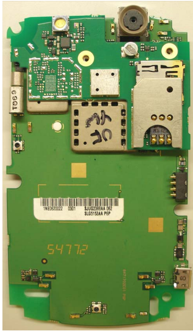
Main and Daughter Boards (Connected Together)
