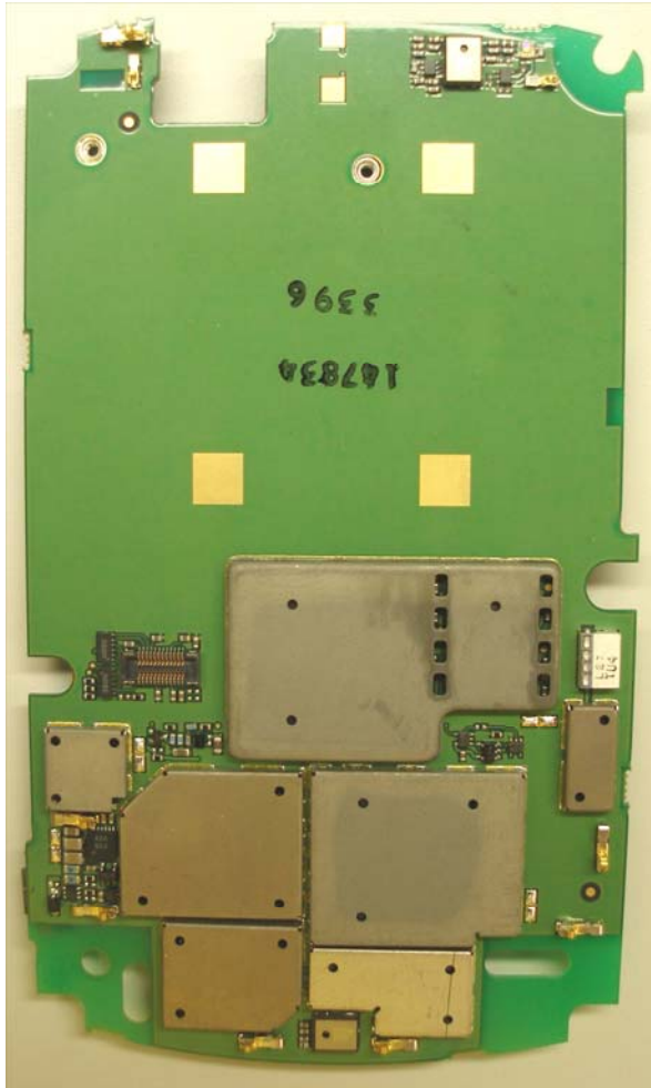
Main Board Back (Without Shields)
