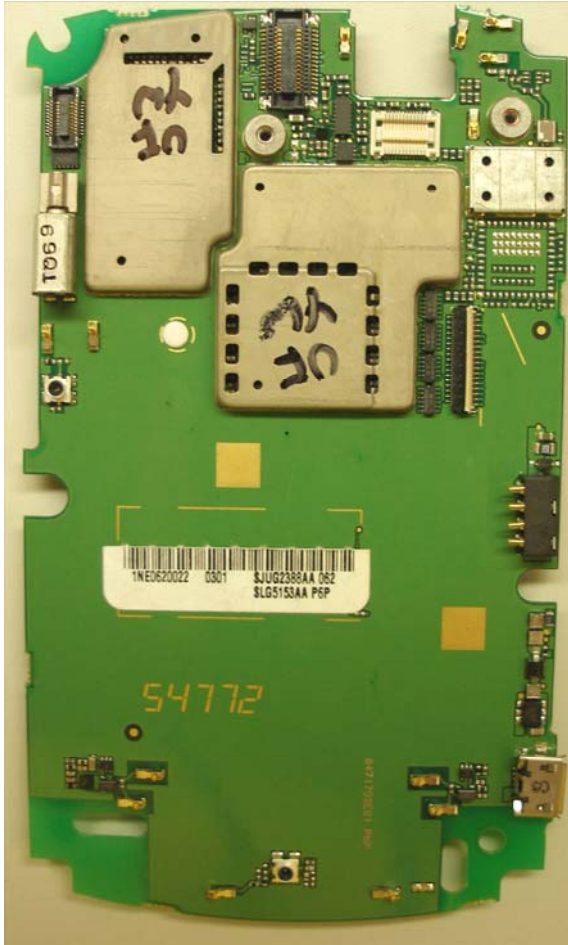
Main Board Front (With Shields)
