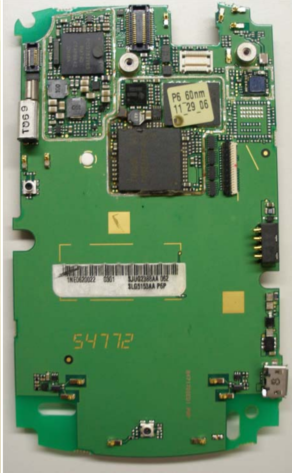
Main Board Front (Without Shields)
