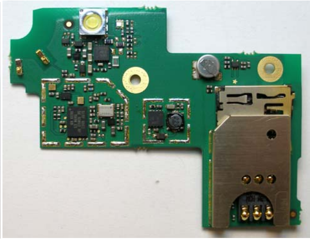
Daughter Board Front (Without Shields and Camera Module)
