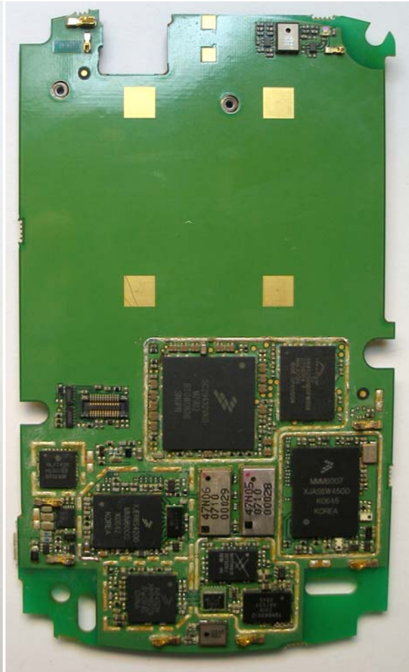
Main Board Back (Without Shields)
