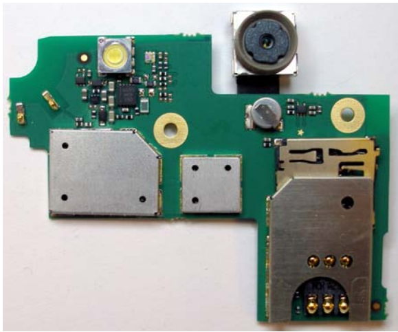
Daughter Board Front (With Shields and Camera Module)
