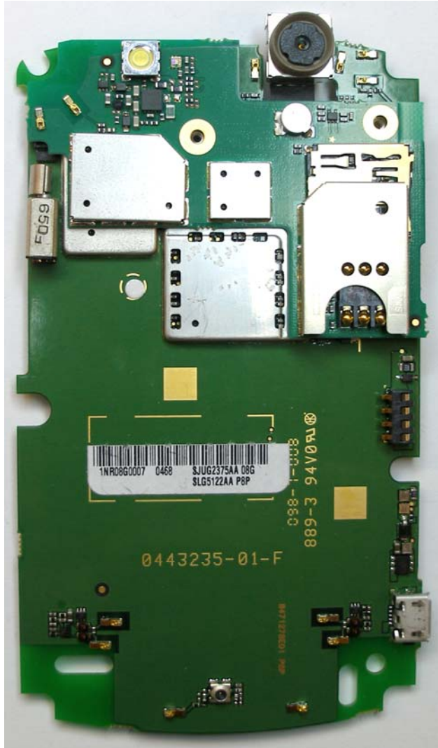
Main and Daughter Boards (Connected Together)
