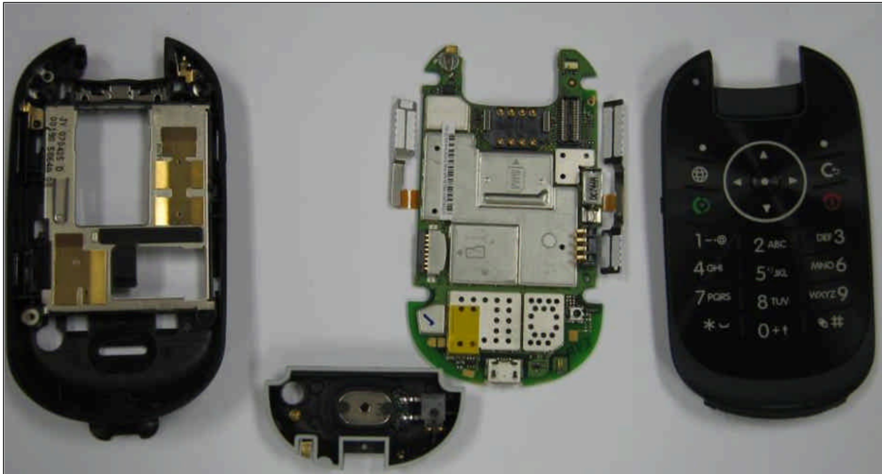
Rear Housing Internal View (Front)
