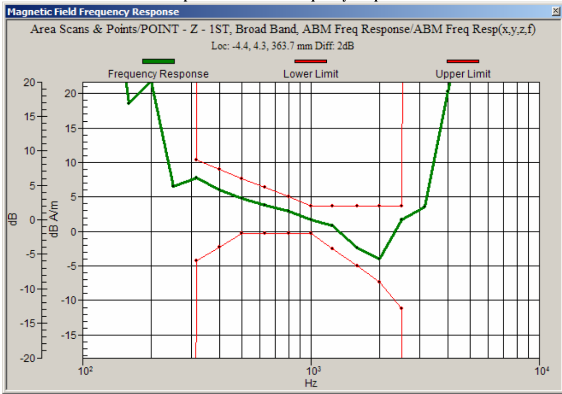
Graph 2: CDMA 800 Frequency Response
