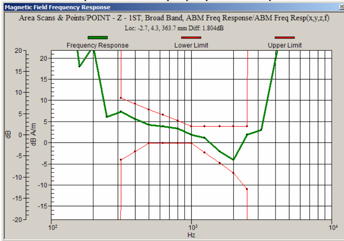
Graph 6: CDMA 1900 Frequency Response with Battery 2
