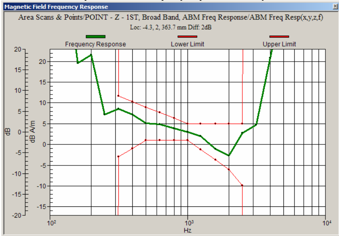
Graph 3: CDMA 800 Frequency Response with Battery 2
