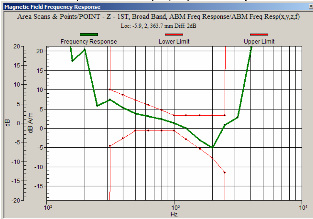
Graph 7: CDMA 1900 Frequency Response with Battery 3
