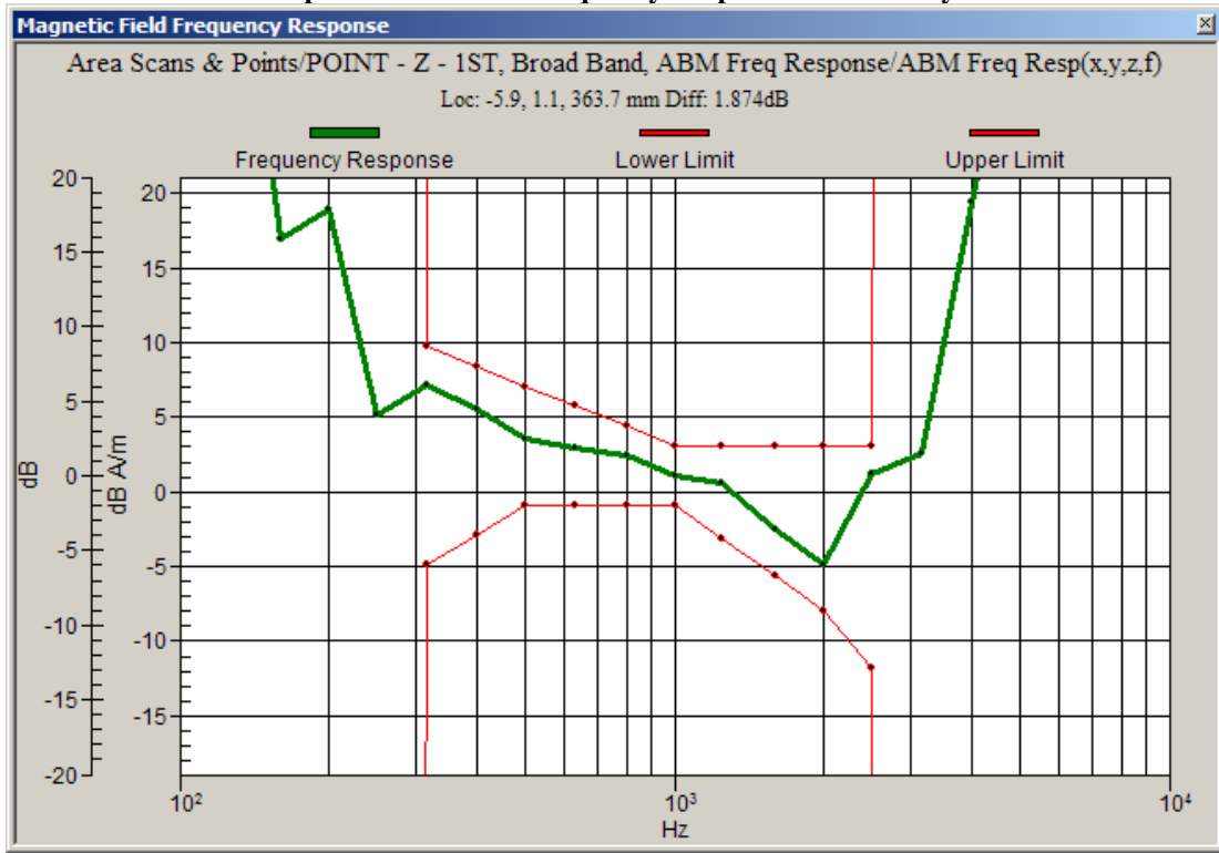
Graph 4: CDMA 800 Frequency Response with Battery 3
