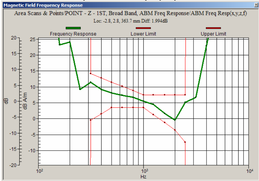
Graph 5: CDMA 1900 Frequency Response
