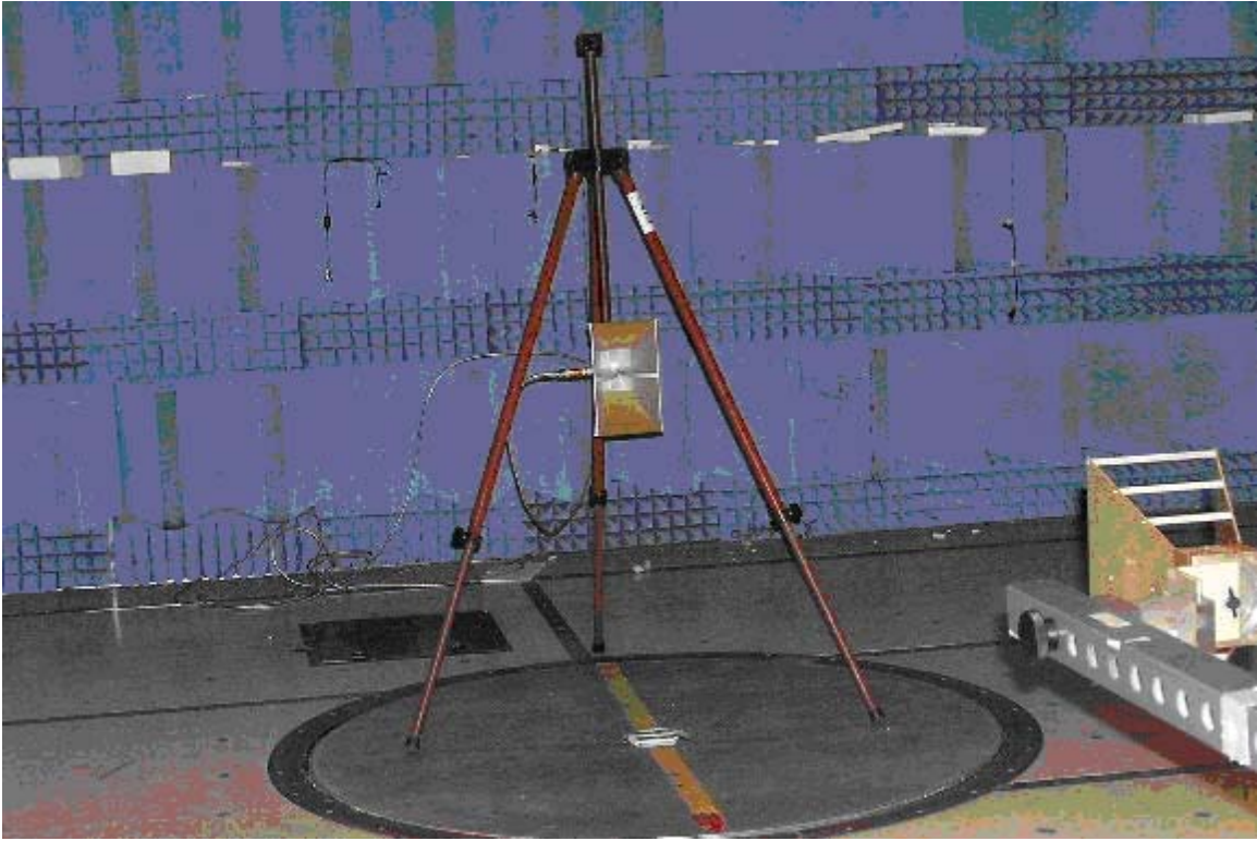
Antenna - Substitution
