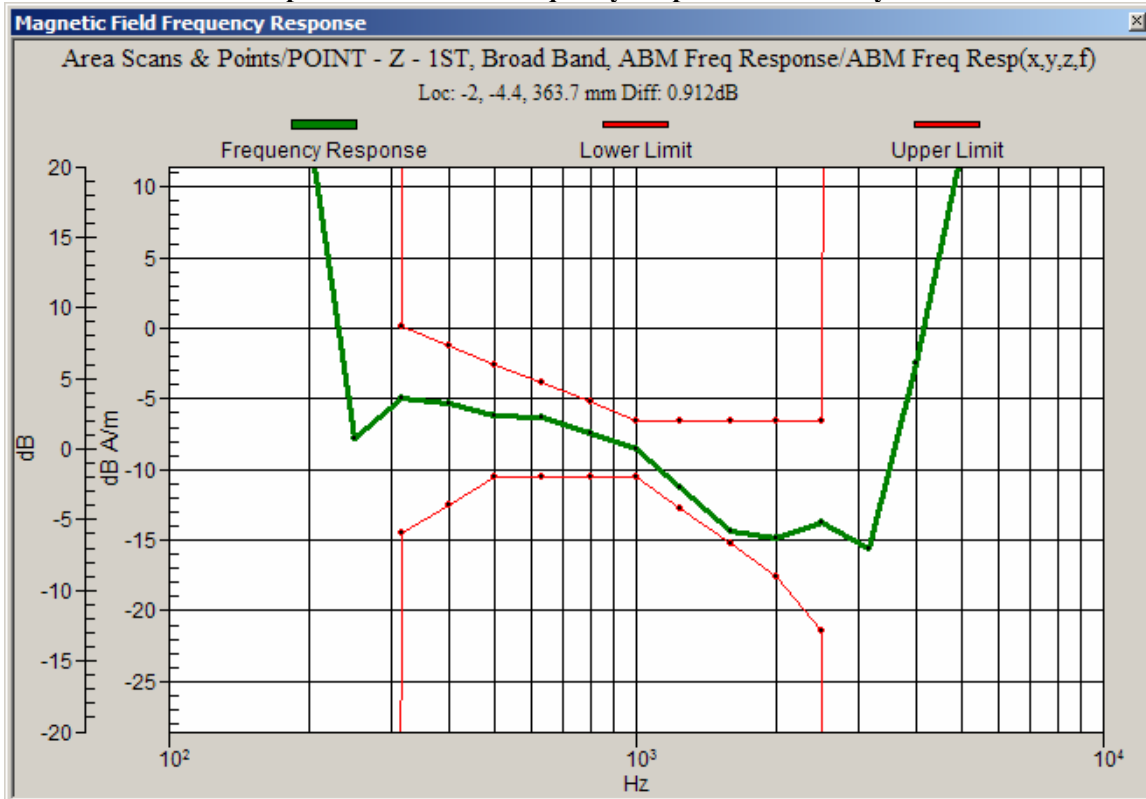
Graph 7: CDMA 1900 Frequency Response with Battery #2
