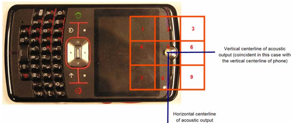
Figure A4-6. Phone Open – 5cm x 5cm grid for Near Field Measurements
