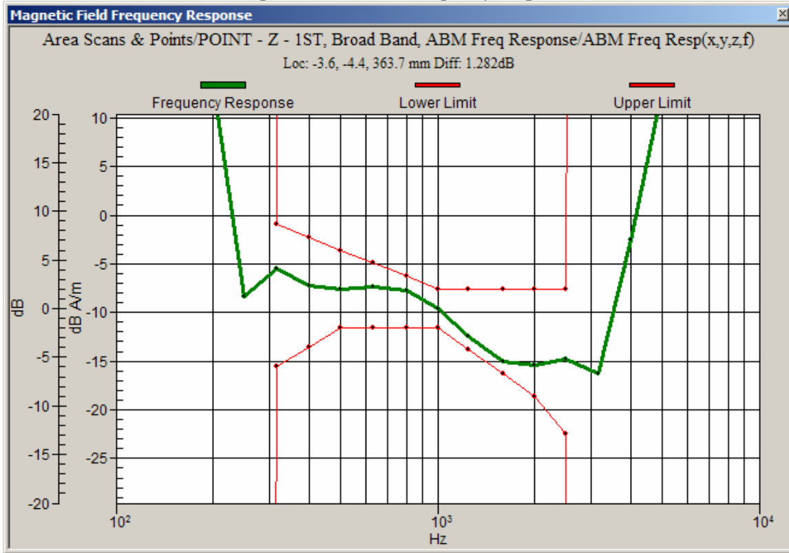
Graph 6: CDMA 1900 Frequency Response
