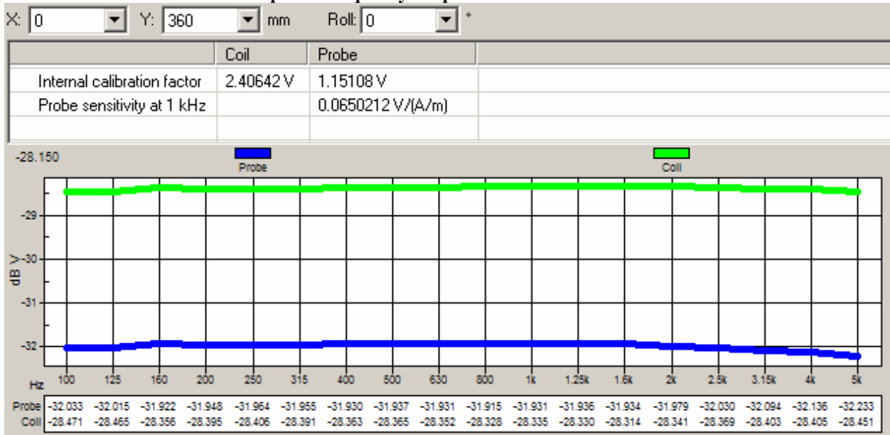
Graph 1: Frequency Response measured in AMCC
