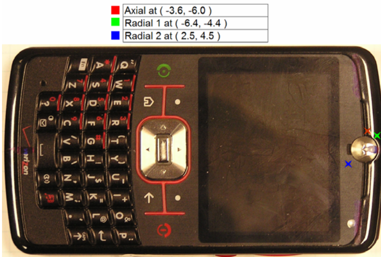
Figure A4-5. Phone Open – Location of Measured Points
