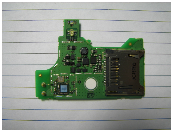
Daughter PCB w/ no shields – Front Side
