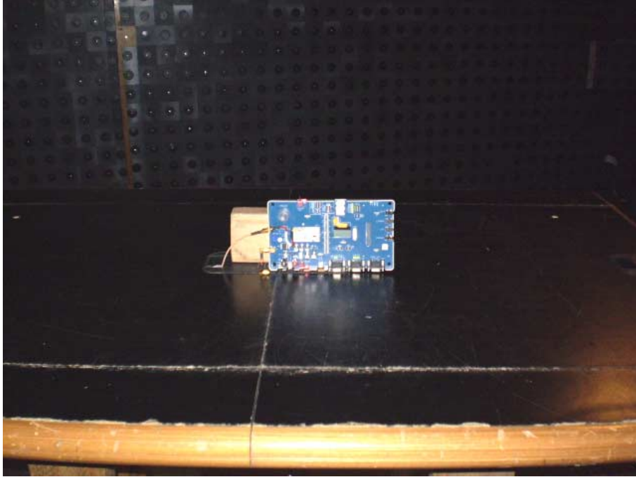
Photograph No.6 Radiated emissions measurement setup in the anechoic chamber EUT close view
