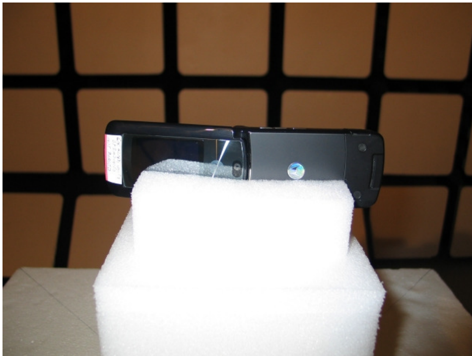
20871-1, IHDT56HN2 placed in test position Y
