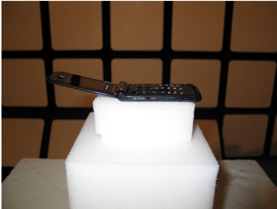
20871-1, IHDT56HN2 placed in test position X
