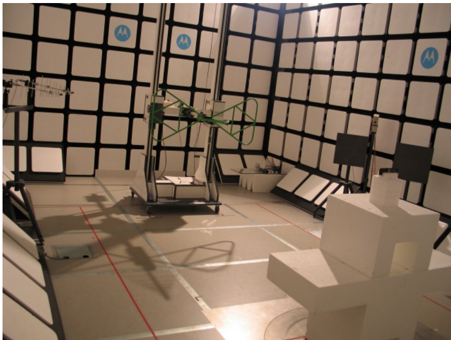
20871-1, IHDT56HN2 setup in semi-anechoic chamber
