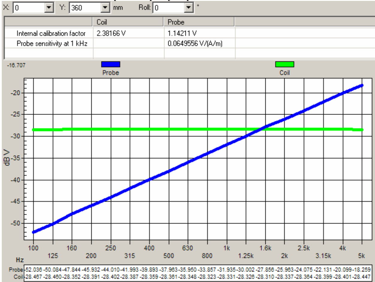
Graph 1: Frequency Response measured in AMCC
