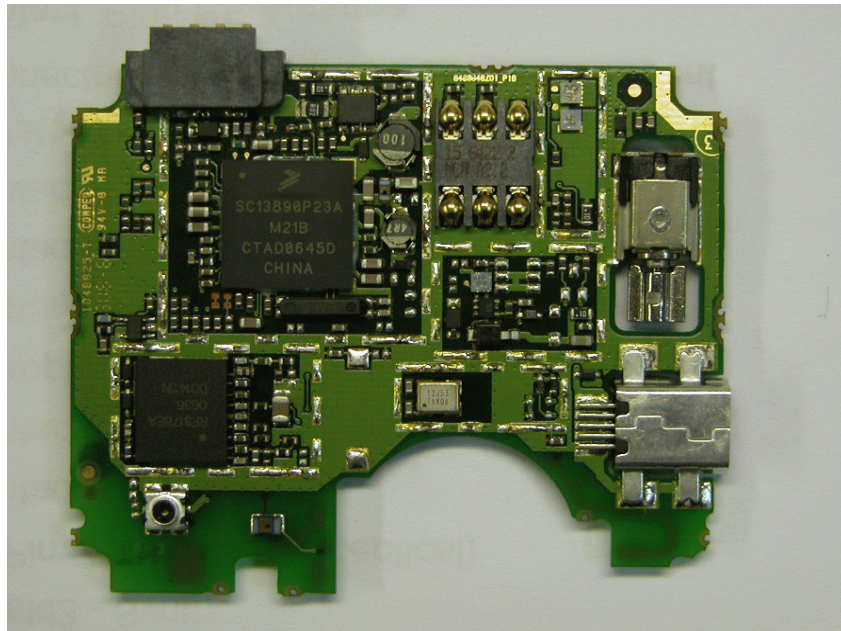
Main Board Bottom Without Shields
