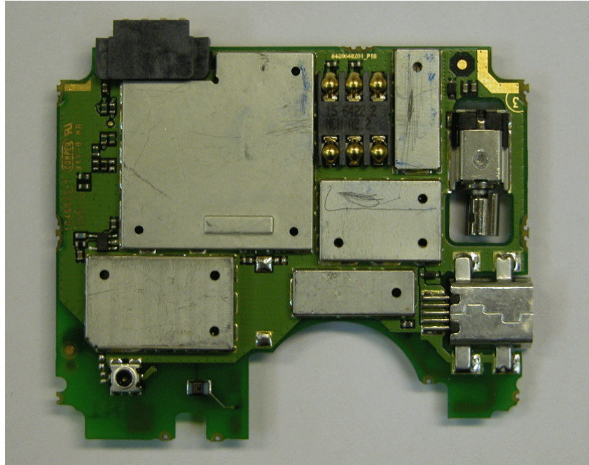
Main Board Bottom With Shields
