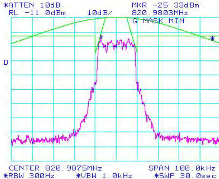
Figure 6a-2.3.2. WiDEN25 800 MHz Band, Quad-QPSK, Minimum Power, Emission Mask G
