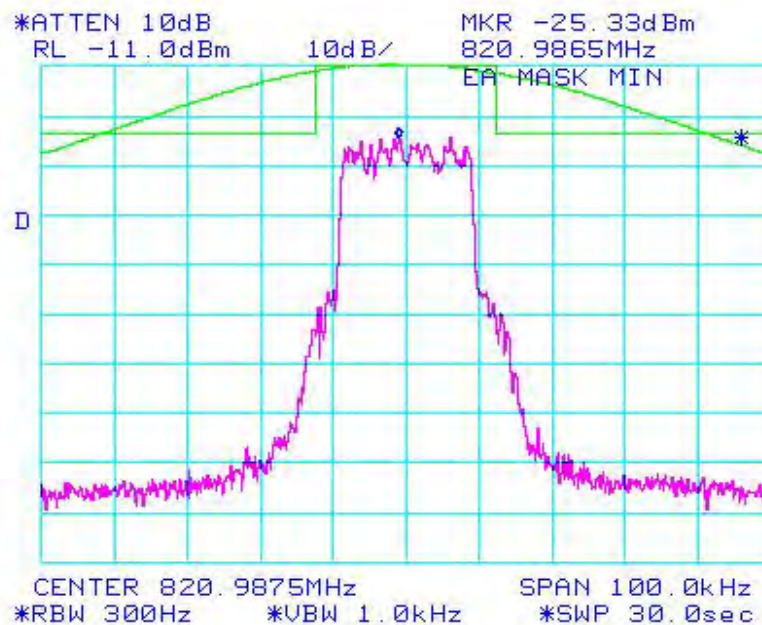
Figure 6a-2.1.12. iDEN 800 MHz Band, QAM64, Minimum Power, EA Emission Mask
