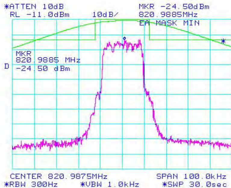
Figure 6a-2.1.8. iDEN 800 MHz Band, QAM16, Minimum Power, EA Emission Mask
