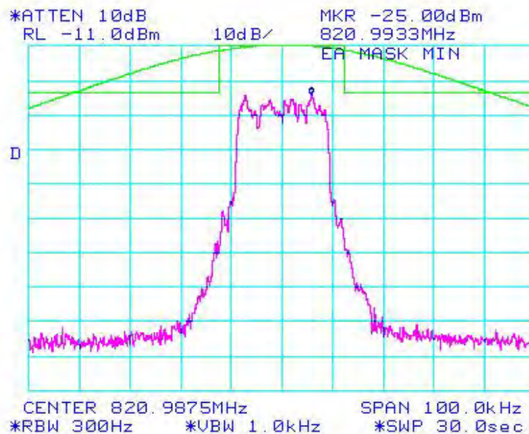
Figure 6a-2.3.4. WiDEN25 800 MHz Band, Quad-QPSK, Minimum Power, EA Emission Mask
