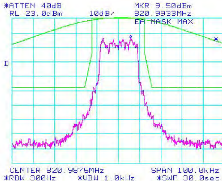
Figure 6a-2.3.3. WiDEN25 800 MHz Band, Quad-QPSK, Maximum Power, EA Emission Mask
