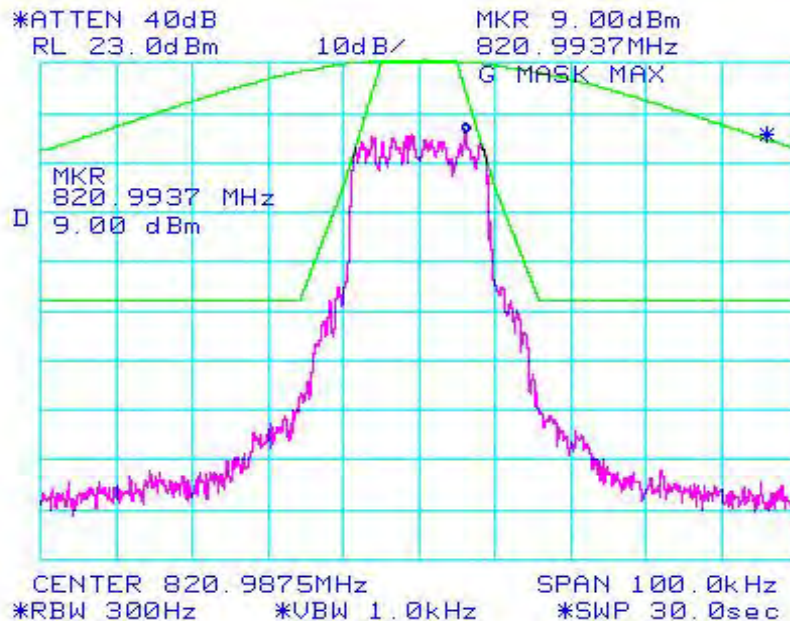
Figure 6a-2.1.9. iDEN 800 MHz Band, QAM64, Maximum Power, Emission Mask G
