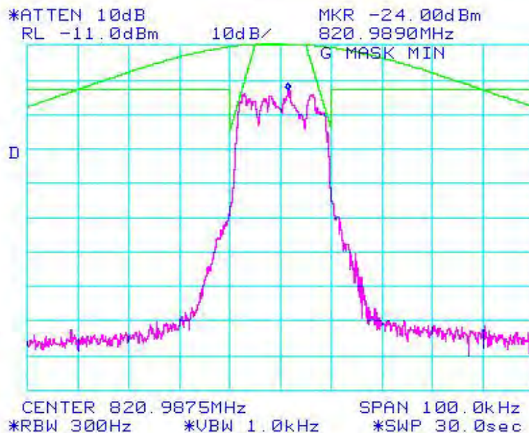
Figure 6a-2.1.2. iDEN 800 MHz Band, QPSK, Minimum Power, Emission Mask G
