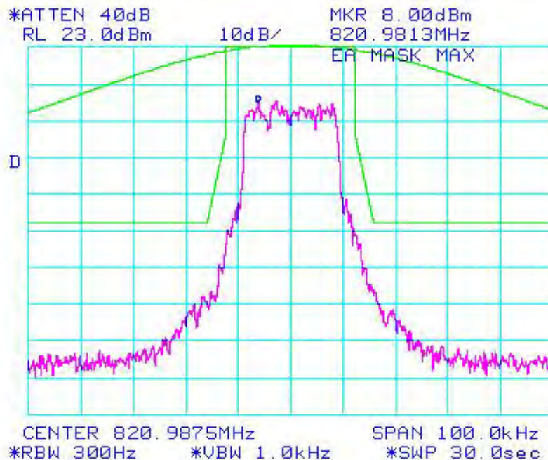
Figure 6a-2.3.11. WiDEN25 800 MHz Band, QAM64, Maximum Power, EA Emission Mask
