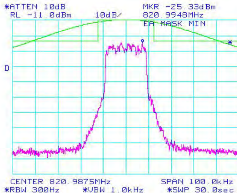
Figure 6a-2.3.8. WiDEN25 800 MHz Band, QAM16, Minimum Power, EA Emission Mask
