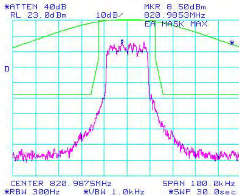
Figure 6a-2.3.7. WiDEN25 800 MHz Band, QAM16, Maximum Power, EA Emission Mask
