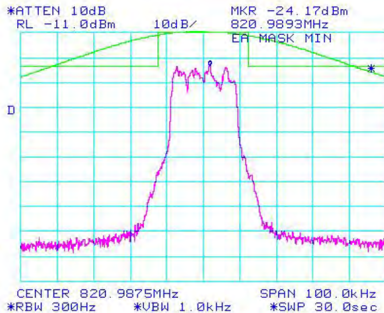
Figure 6a-2.1.4. iDEN 800 MHz Band, QPSK, Minimum Power, EA Emission Mask
