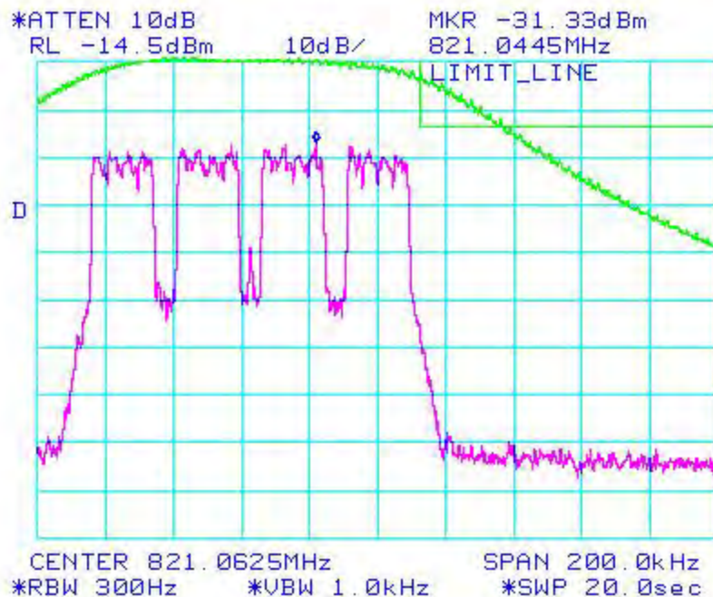
Figure 6a-2.6.2. WiDEN100 800 MHz Band, Quad-QPSK, Minimum Power, EA Emission Mask
