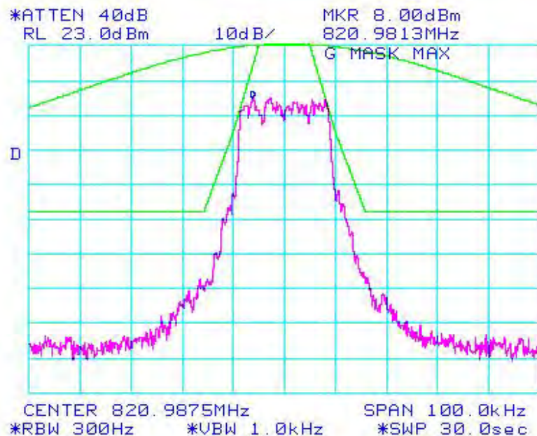
Figure 6a-2.3.9. WiDEN25 800 MHz Band, QAM64, Maximum Power, Emission Mask G
