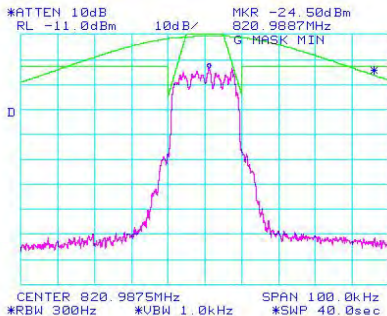
Figure 6a-2.1.6. iDEN 800 MHz Band, QAM16, Minimum Power, Emission Mask G
