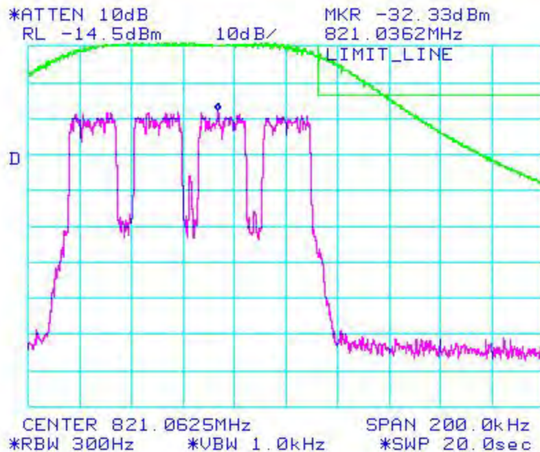
Figure 6a-2.6.4. WiDEN100 800 MHz Band, QAM16, Minimum Power, EA Emission Mask
