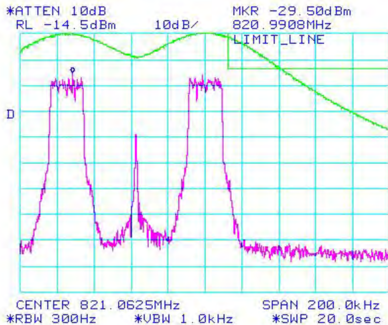
Figure 6a-2.7.4. WiDEN50_Split 800 MHz Band, QAM16, Minimum Power, EA Emission Mask
