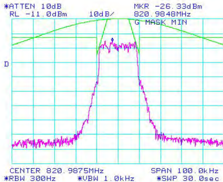
Figure 6a-2.3.10. WiDEN25 800 MHz Band, QAM64, Minimum Power, Emission Mask G
