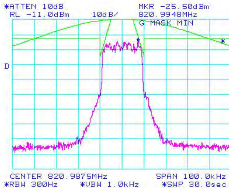
Figure 6a-2.3.6. WiDEN25 800 MHz Band, QAM16, Minimum Power, Emission Mask G
