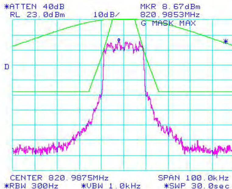
Figure 6a-2.3.5. WiDEN25 800 MHz Band, QAM16, Maximum Power, Emission Mask G
