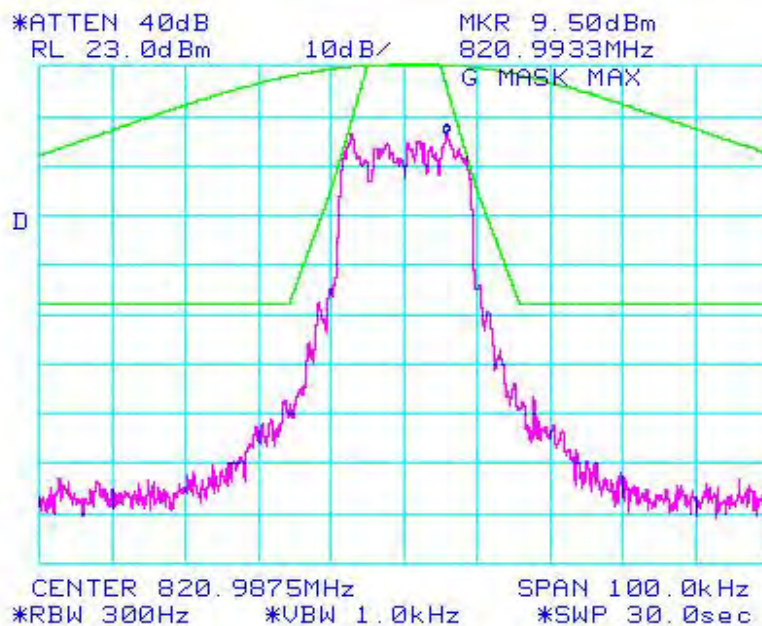
Figure 6a-2.3.1. WiDEN25 800 MHz Band, Quad-QPSK, Maximum Power, Emission Mask G
