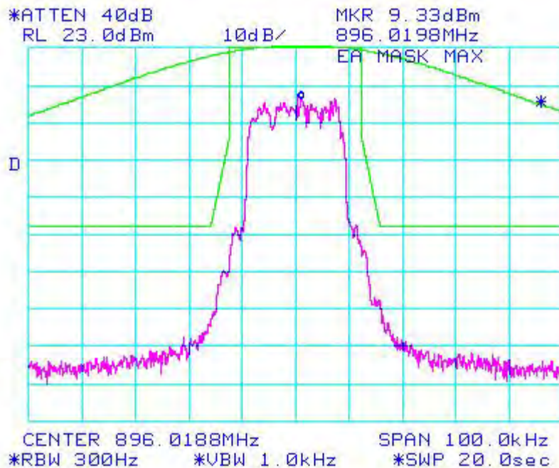
Figure 6a-2.2.3. iDEN 900 MHz Band, QAM16, Maximum Power, EA Emission Mask
