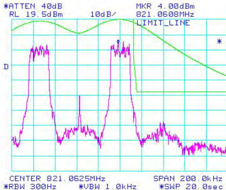
Figure 6a-2.7.3. WiDEN50_Split 800 MHz Band, QAM16, Maximum Power, EA Emission Mask
