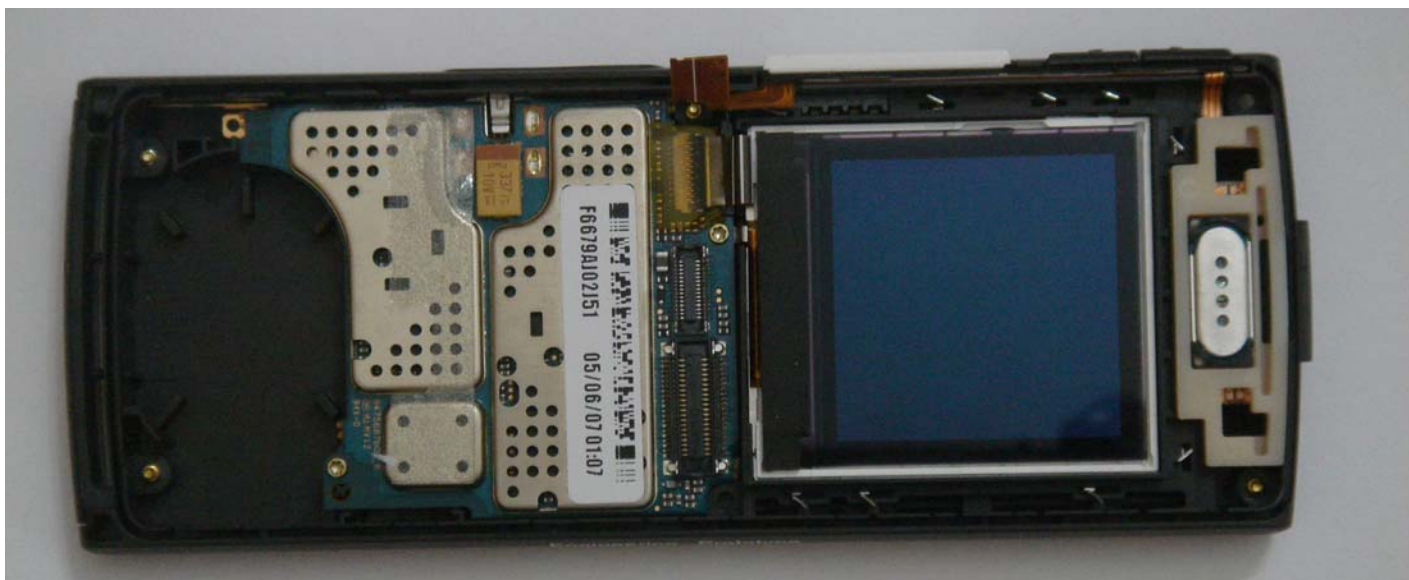
Photograph 9-2: Front side view of radio product PC Board with Keypad PC Board detached
