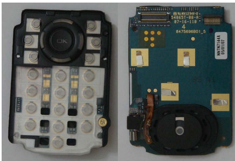
Photograph 9-4: Front and Back side view of keypad PC Board.
