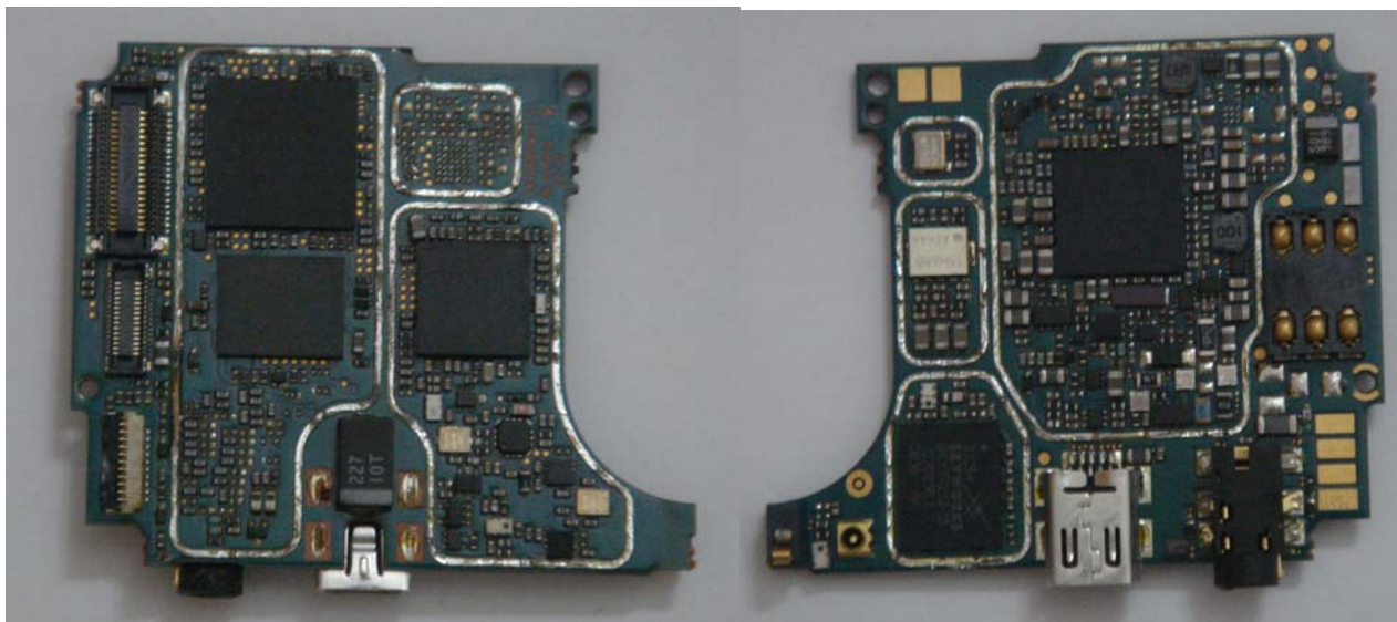
Photograph 9-3: Front and Back side view of radio PC Board, without shields.
