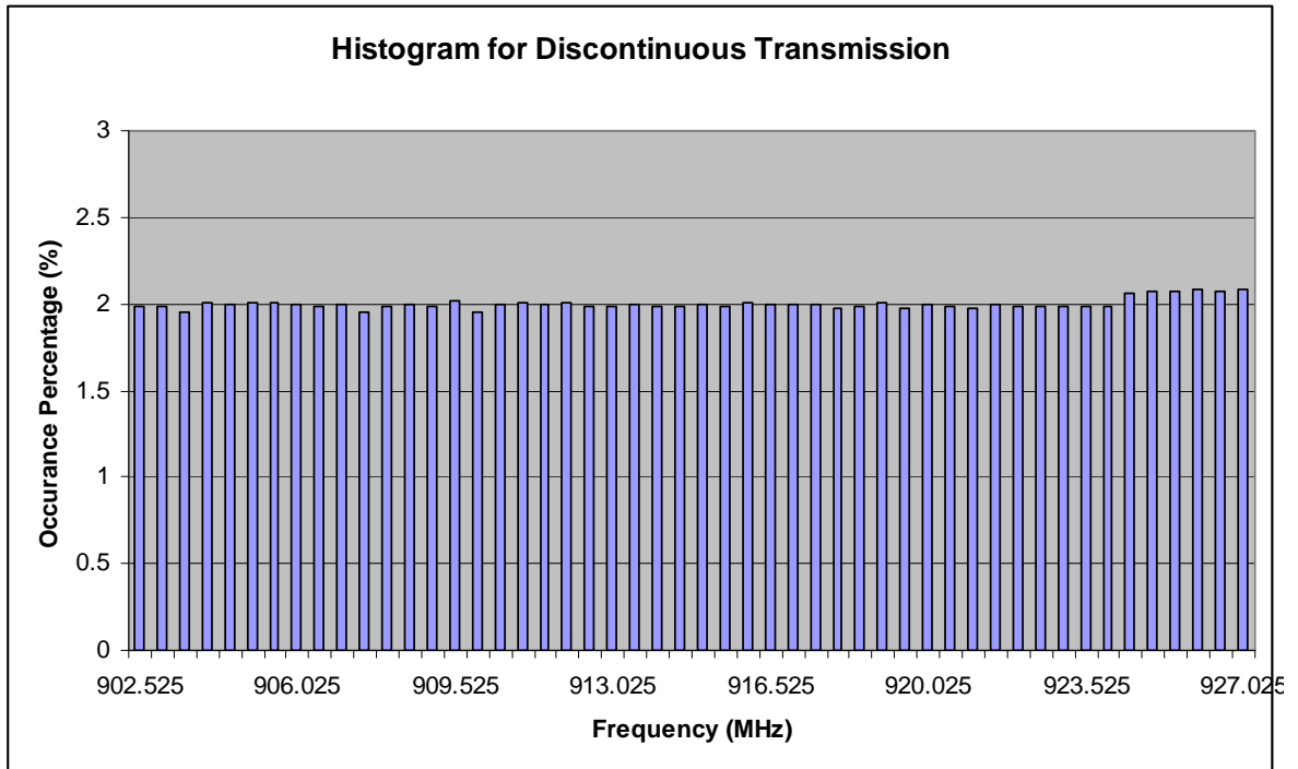
Figure 6b-2.7.1. Histogram for MOTotalk ISM Band Discontinuous Transmission
