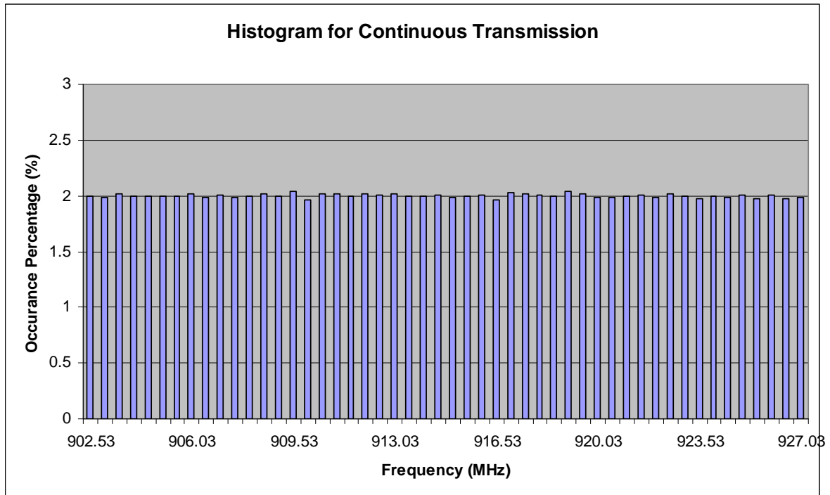
Figure 6b-2.6.1. Histogram for MOTOtalk ISM Band Continuous Transmission
