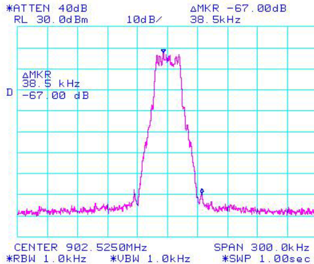
Figure 6b-2.2.3 MOTOtalk ISM band occupied bandwidth with frequency span of 300 kHz with hopping function disabled at center frequency 902.525 MHz.
