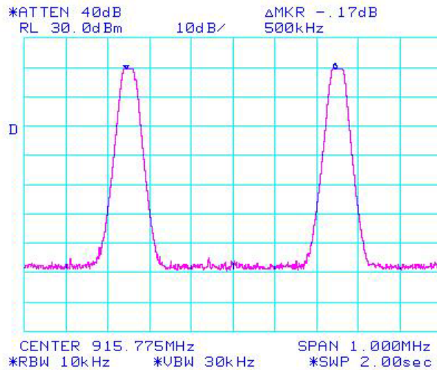
Figure 6b-2.1.1. Plot of MOTotalk ISM Band adjacent channel separation within a hop set
