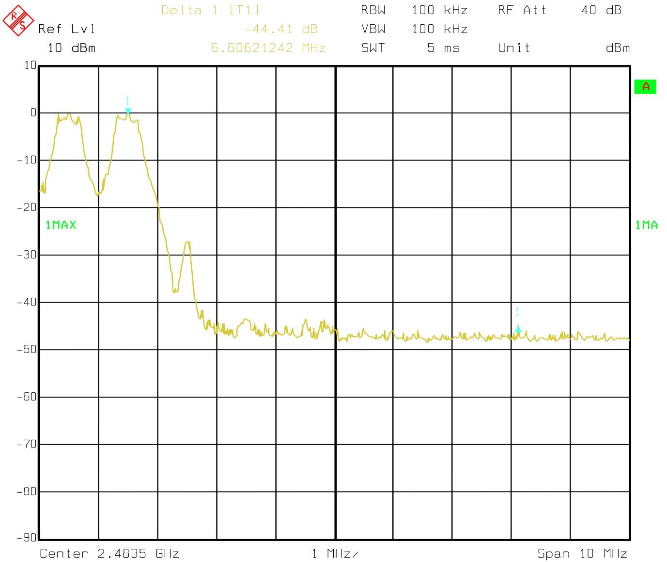
Figure 6d.6-4: Plot of upper band-edge conducted emissions with hopping enabled.
