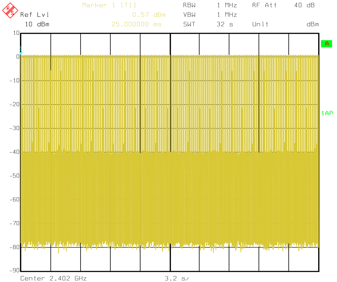
Figure 6d.4-1: Plot of dwell time over 32 second period
