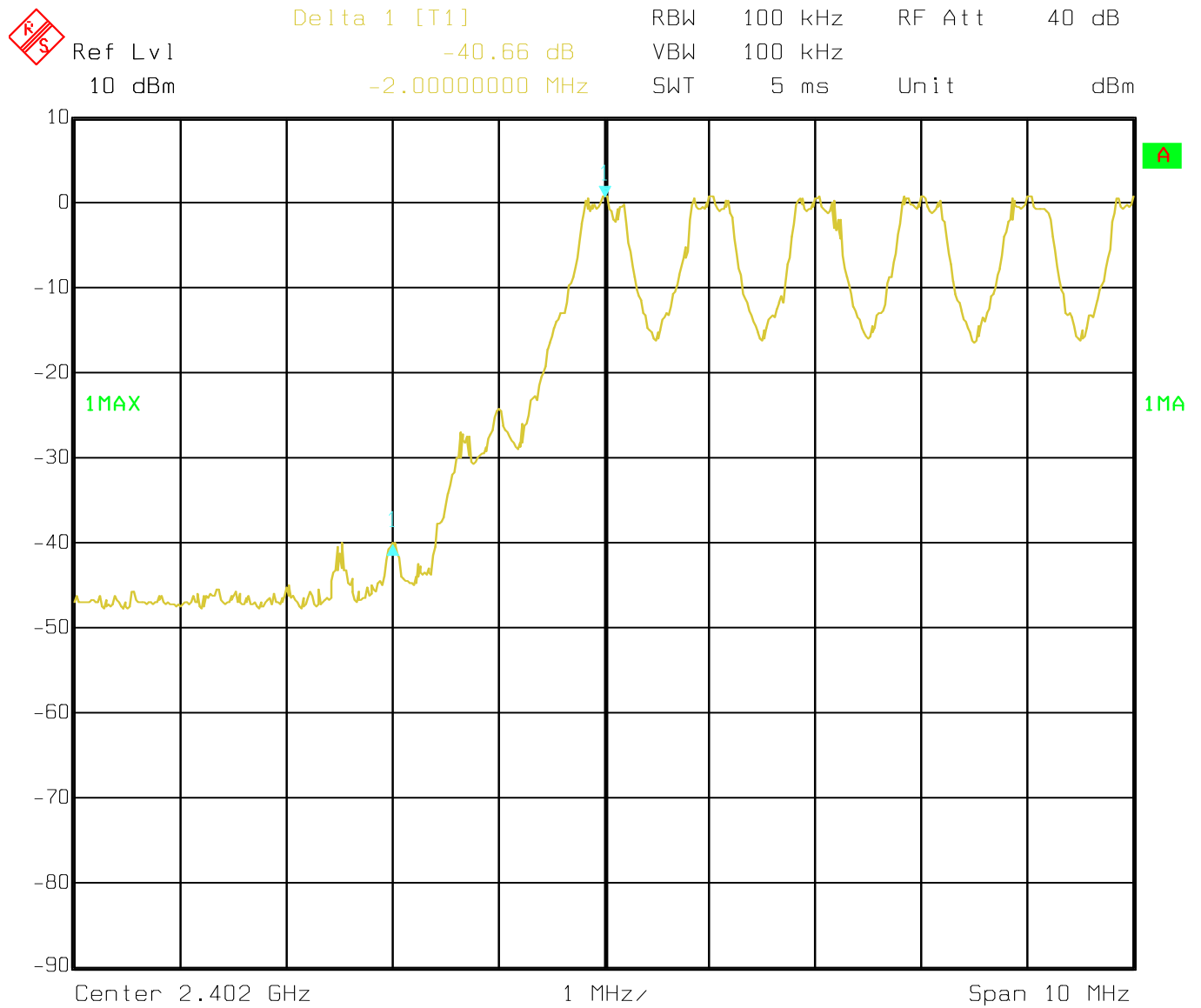
Figure 6d.6-3: Plot of lower band-edge conducted emissions with hopping enabled.
