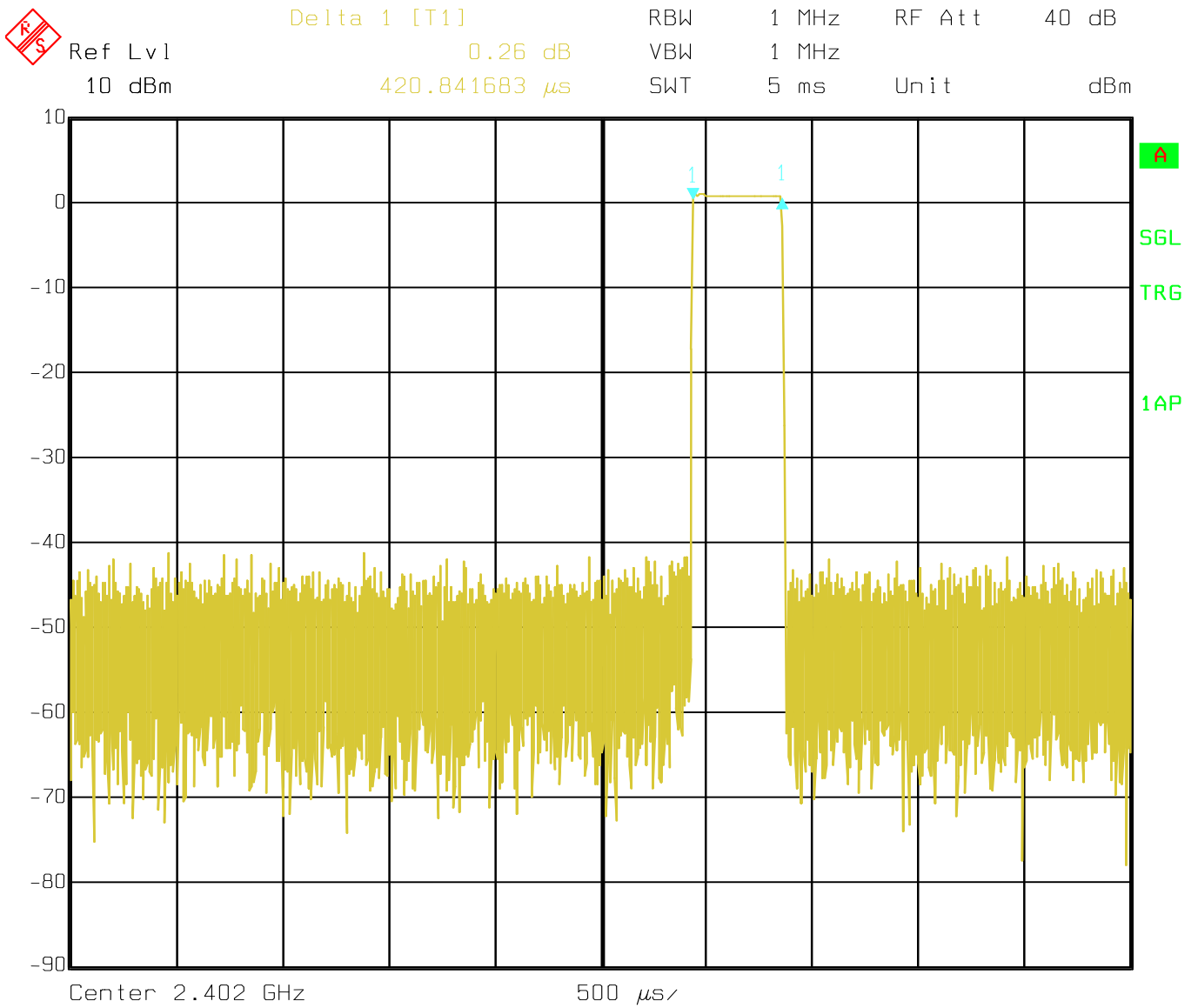
Figure 6d.4-3: Plot of dwell time over 5 ms period.
