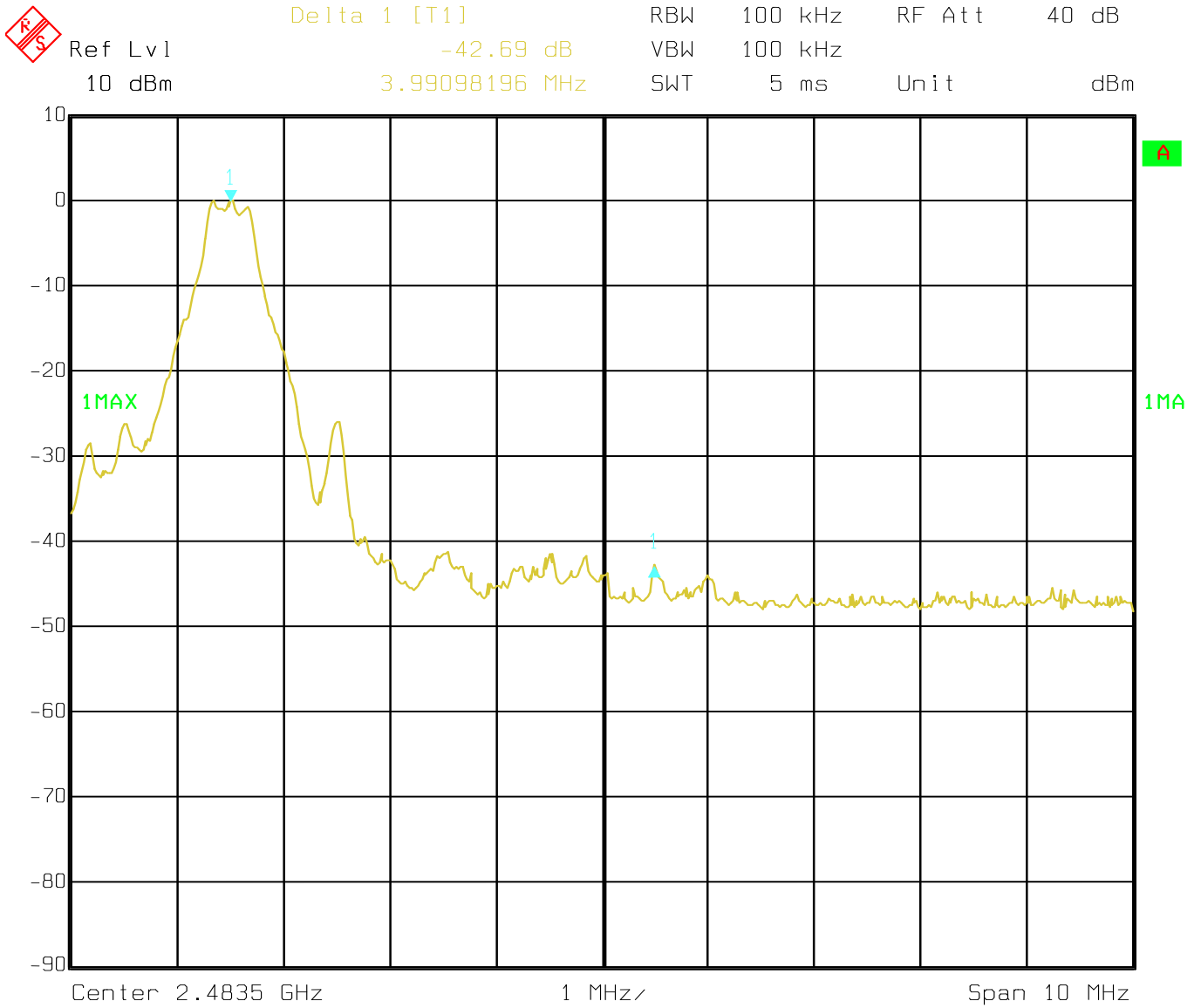
Figure 6d.6-2: Plot of upper band-edge conducted emissions with hopping disabled.
