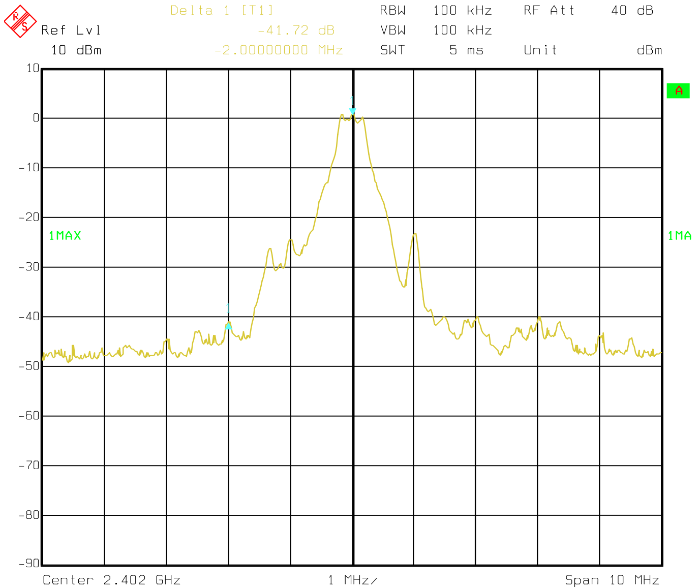
Figure 6d.6-1: Plot of lower band-edge conducted emissions with hopping disabled
