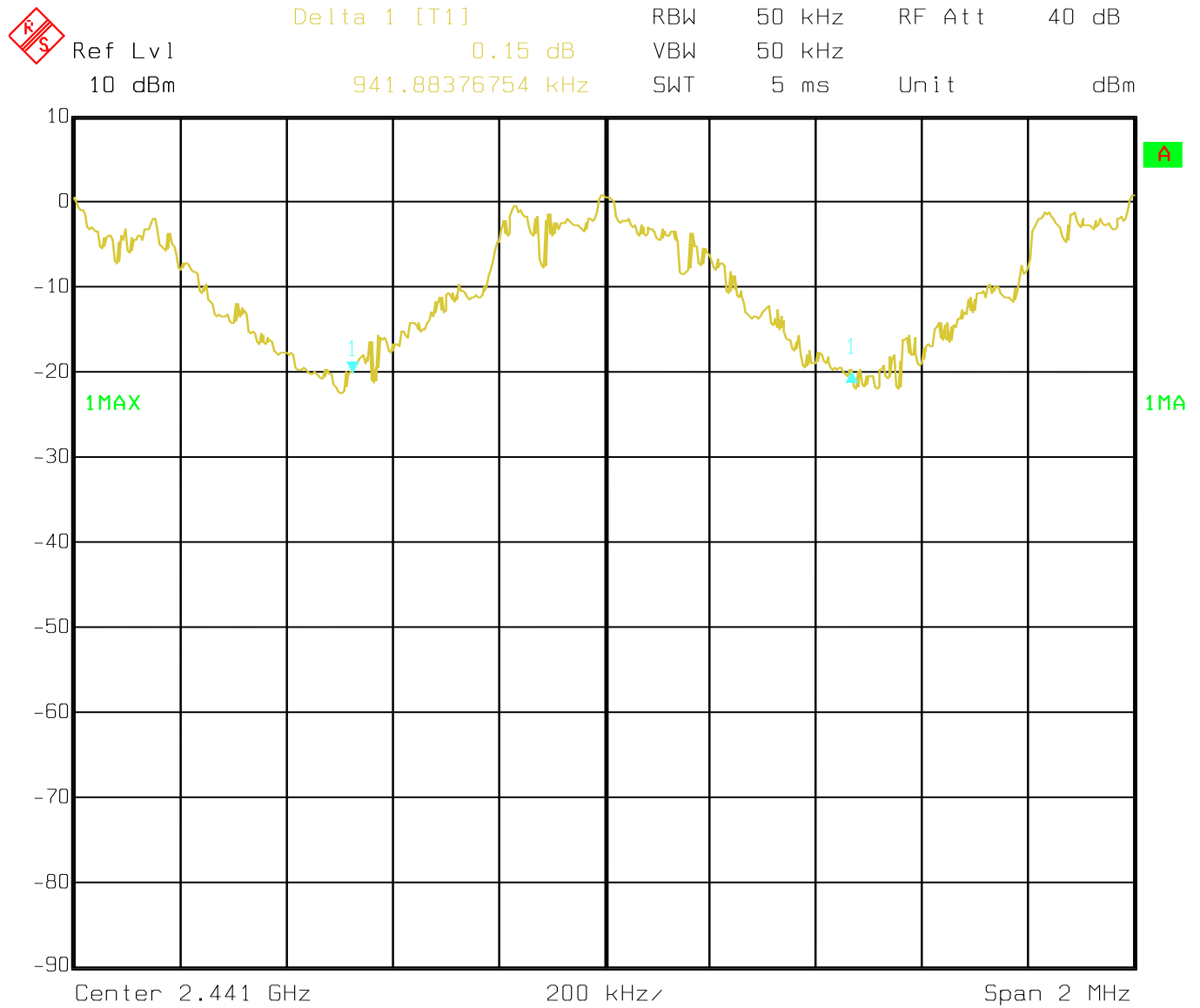
Figure 6d.2-1: Plot of 20 – dB bandwidth
