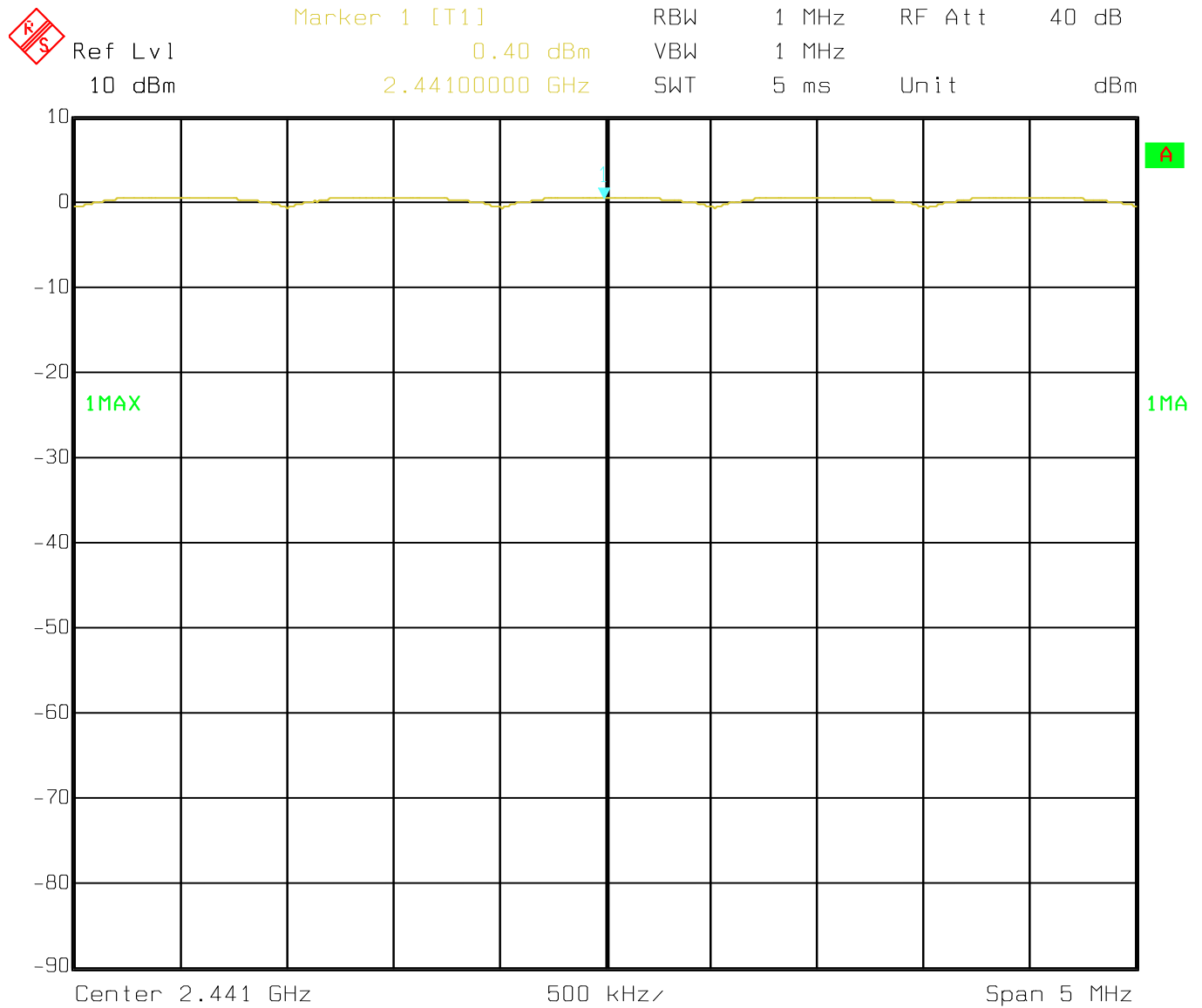
Figure 6d.5-1: Plot of peak output power
