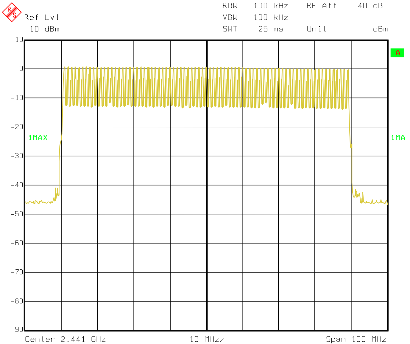
Figure 6d.3-1: Plot of number of Bluetooth hopping frequencies
