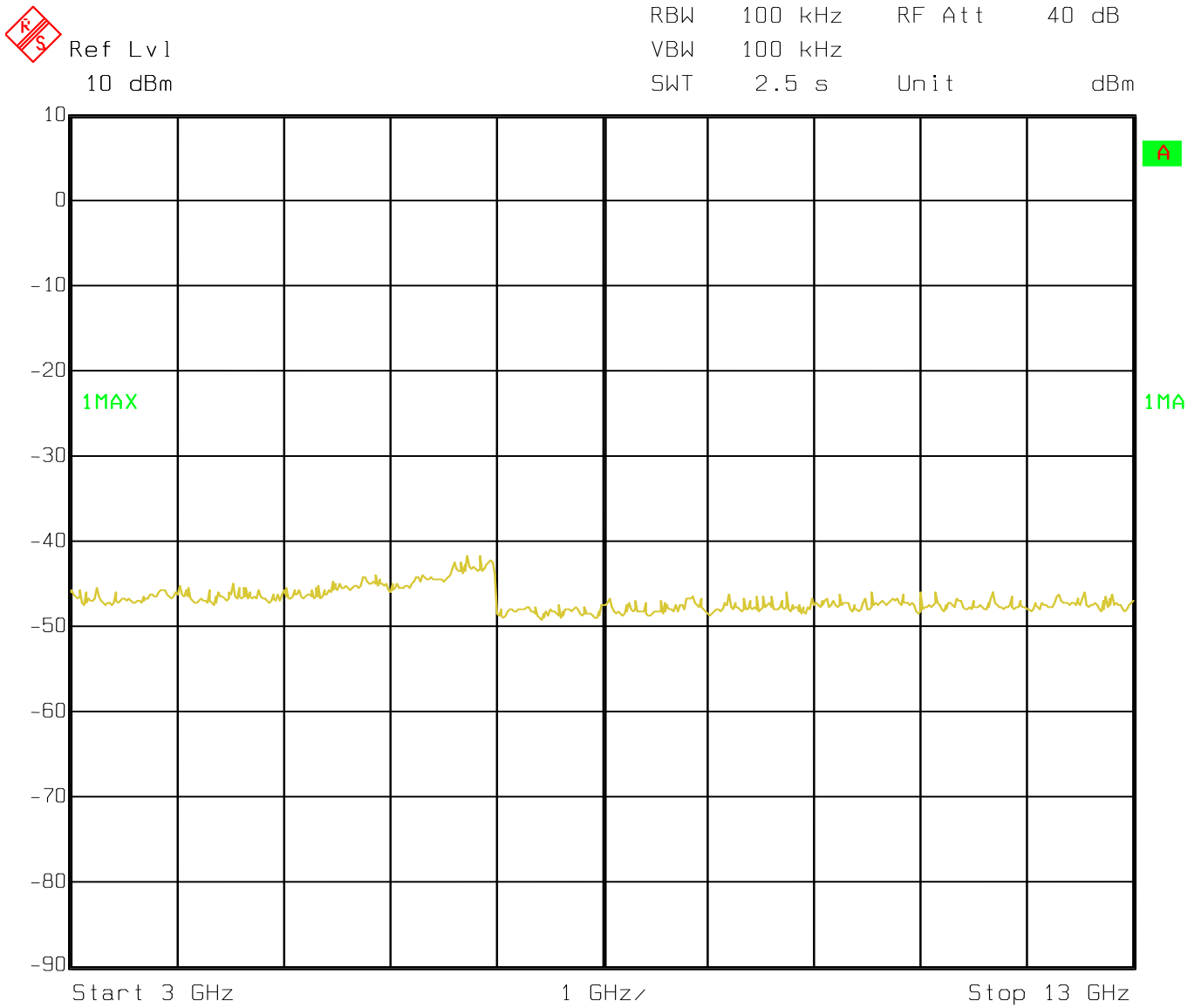
Figure 6d.7-2: Plot of spurious conducted emissions 3 GHz – 13 GHz.
