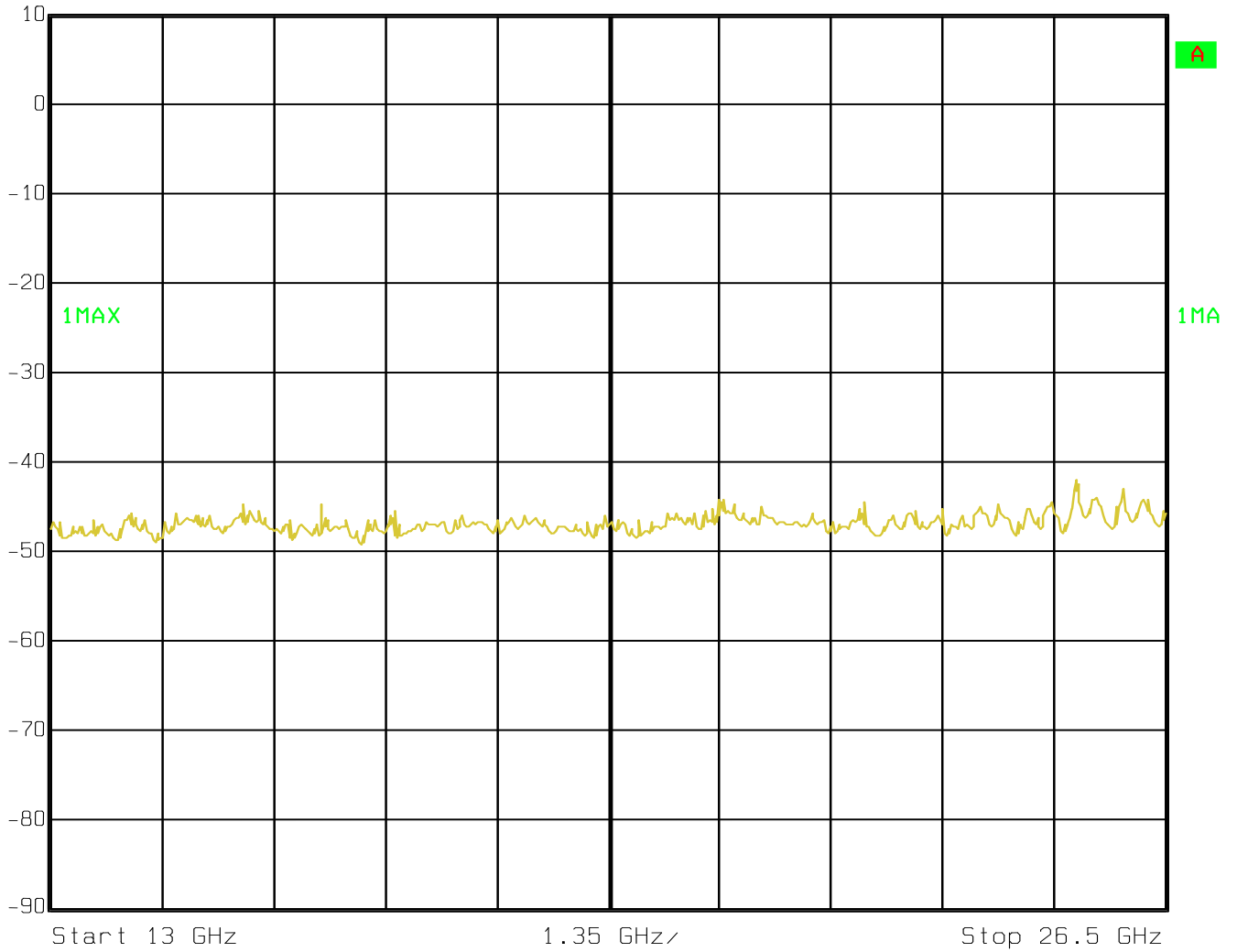
Figure 6d.7-3: Plot of spurious conducted emissions 13 GHz – 26.5 GHz.
