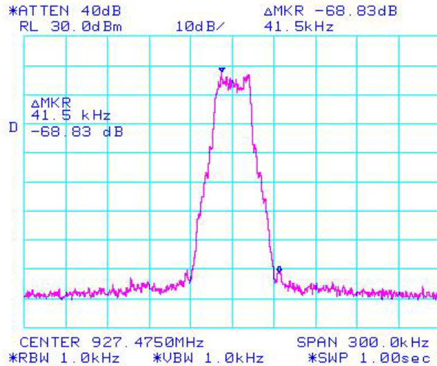
Figure 6c.2.2.7 MOTotalk ISM band occupied bandwidth with frequency span of 300 kHz with hopping function disabled, at center frequency 927.475.
