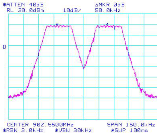
Figure 6c.2.2.2. Adjacent hop set separation with spectrum analyzer center frequency at 902.55 MHz.
