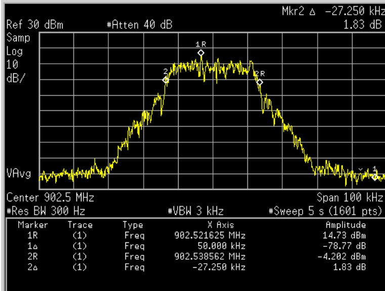
Figure 6c.2.2.1 Spectrum analyzer plot of MOTotalk ISM Band 8-FSK traffic channel signal’s 99% bandwidth at center frequency 902.525 MHz, with hopping function disabled.
