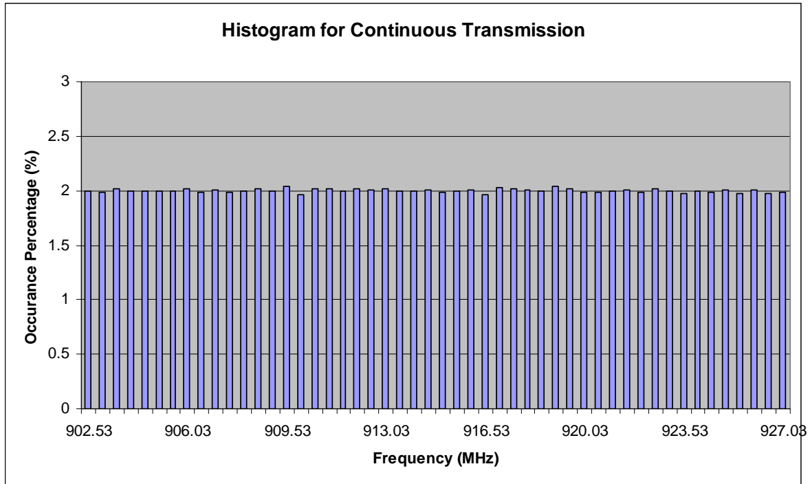
Figure 6c.2.6.1. Histogram of MOTotalk ISM Band Continuous Transmission.
