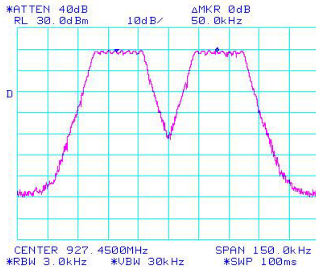
Figure 6c.2.2.6. Adjacent hop set separation with spectrum analyzer center frequency 927.5 MHz.
