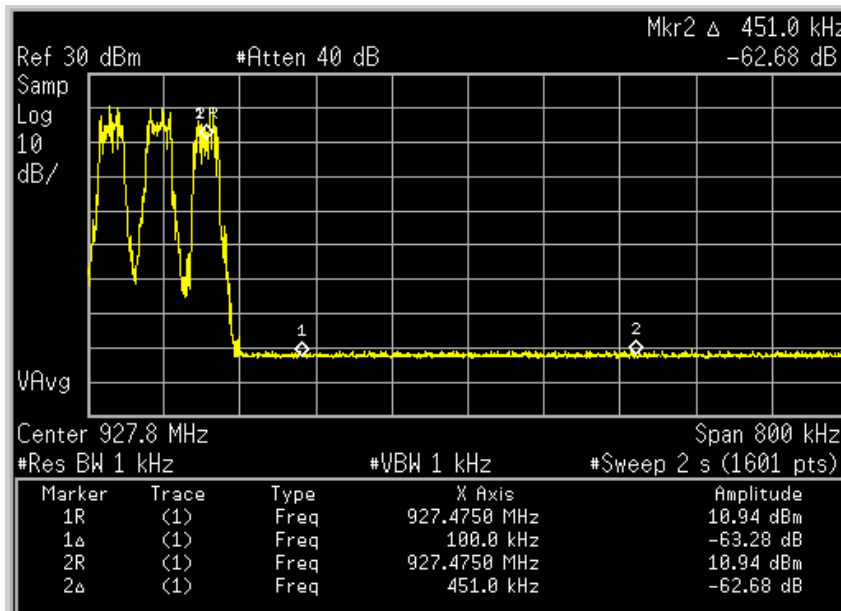
Figure 6c.2.2.8. Out-of-band transmitter spurious emissions high band edge, with hopping function enabled.
