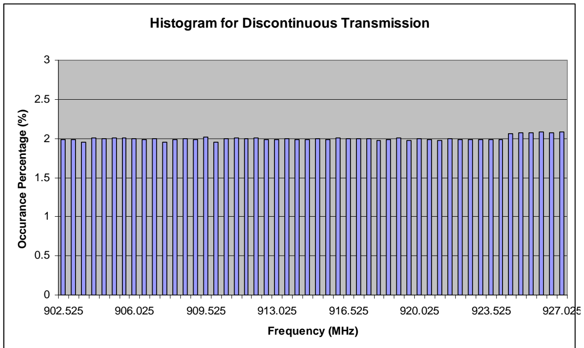
Figure 6c.2.7.1. Histogram of MOTotalk ISM Band Discontinuous Transmissions.
