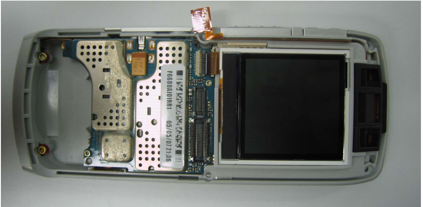
Photograph 9-1: Front side view of radio product PC Board with Keypad PC Board detached
