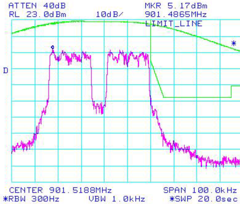
Figure 6b.2.3.1. WiDEN 50 NBPCS Band, QPSK; Occupied Bandwidth
