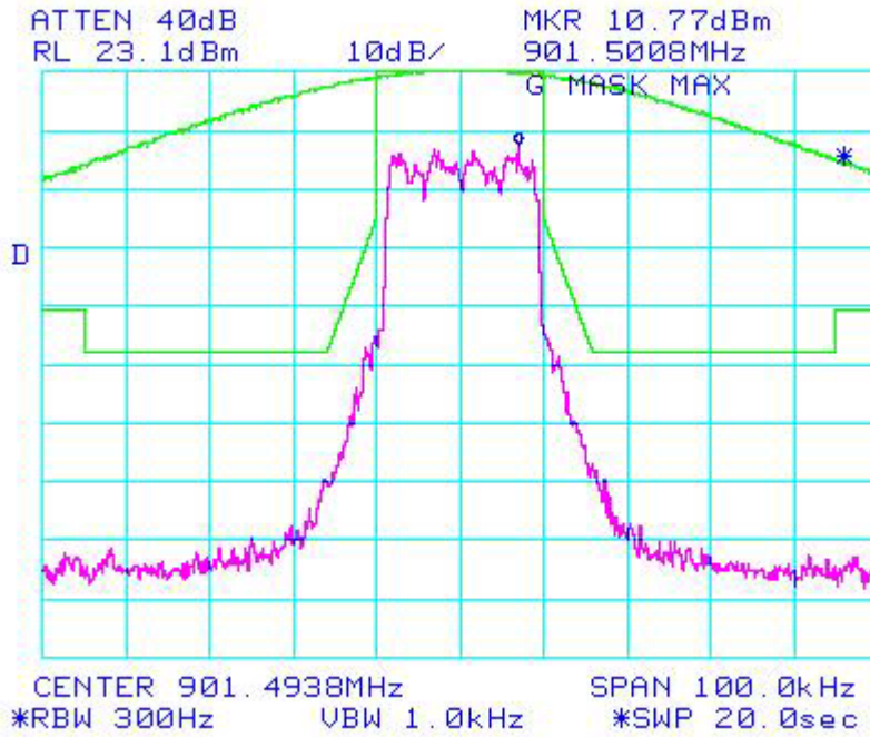
Figure 6b.2.2.1. WiDEN 25 NBPCS Band, QPSK, Occupied Bandwidth
