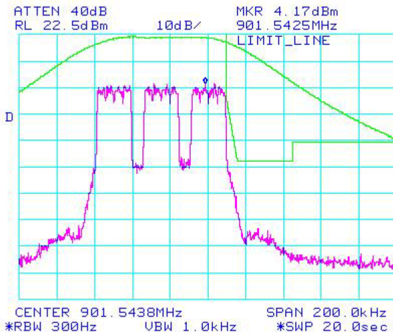
Figure 6b.2.4.2. WiDEN 75 NBPCS Band, Quad-16 QAM; Occupied Bandwidth
