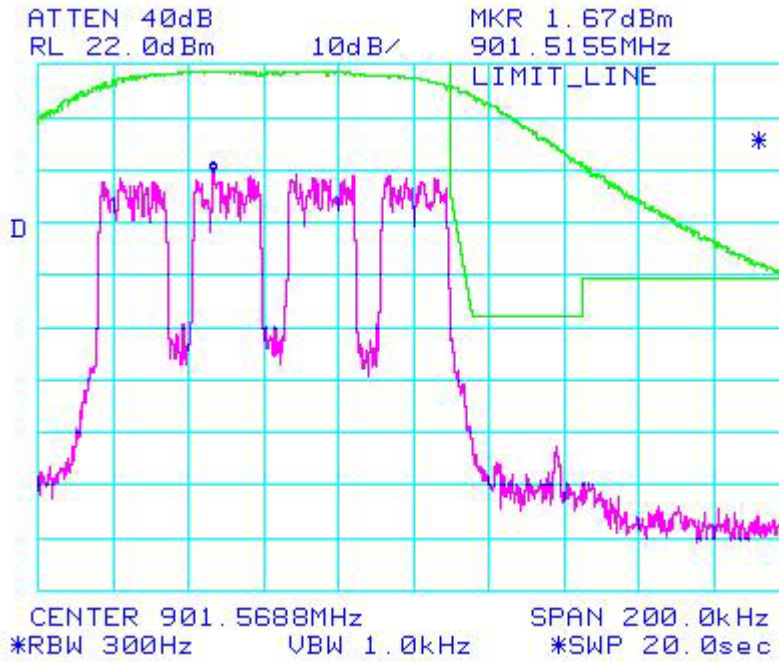
Figure 6b.2.5.1. WiDEN 100 NBPCS Band, QPSK; Occupied Bandwidth
