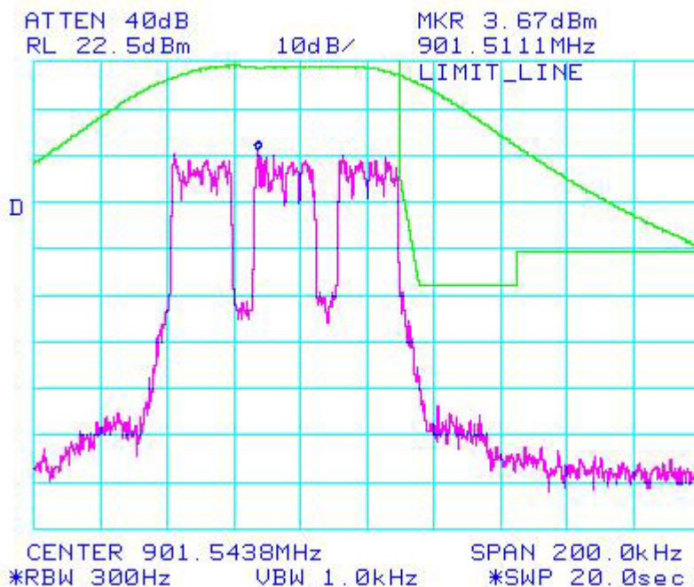
Figure 6b.2.4.1. WiDEN 75 NBPCS MHz Band, QPSK; Occupied Bandwidth
