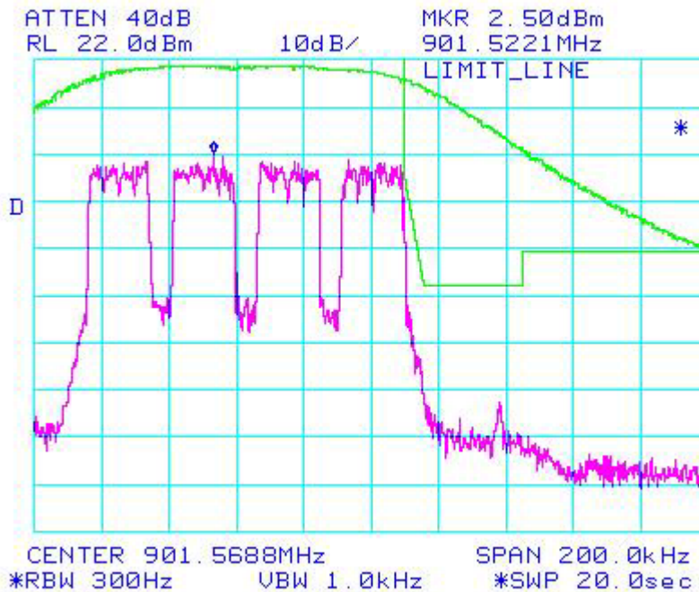
Figure 6b.2.5.2. WiDEN 100 NBPCS Band, Quad-16 QAM; Occupied Bandwidth
