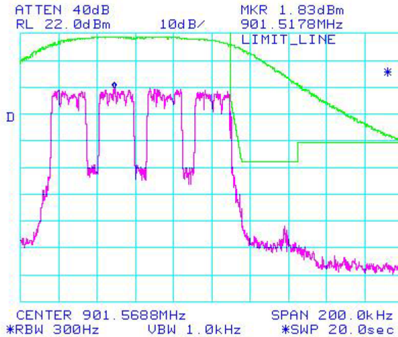
Figure 6b.2.5.3.15. WiDEN 100 NBPCS Band, Quad- 64 QAM; Occupied Bandwidth
