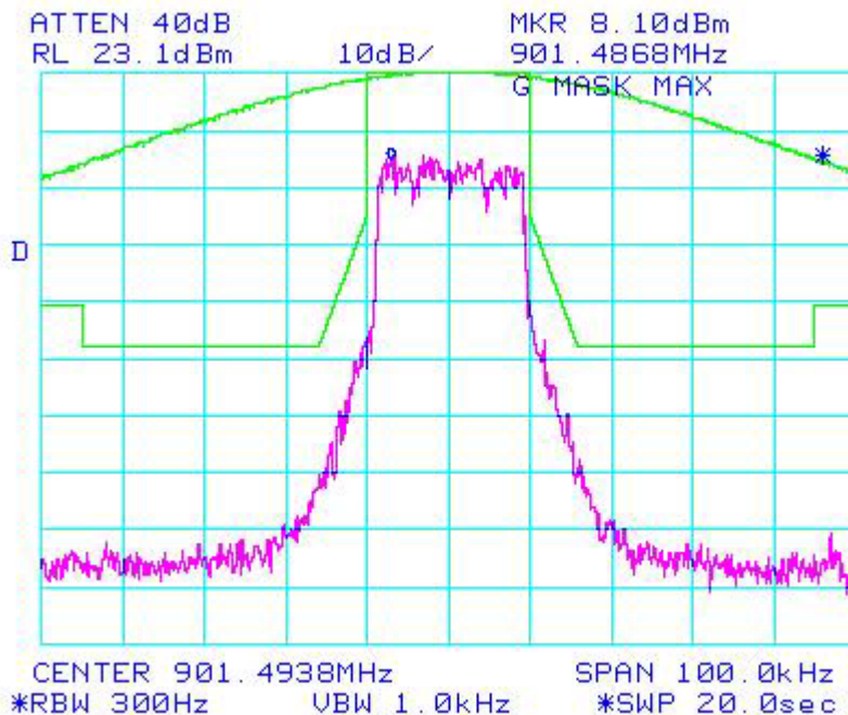
Figure 6b.2.2.3. WiDEN 25 NBPCS Band, Quad- 64 QAM; Occupied Bandwidth
