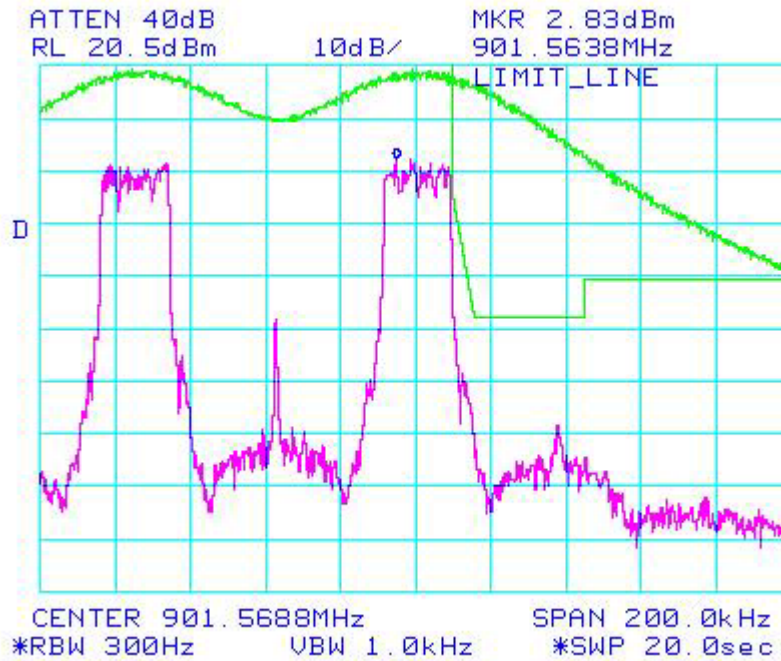
Figure 6b.2.6.318. WiDEN50 Split NBPCS Band, Quad- 64 QAM; Occupied Bandwidth
