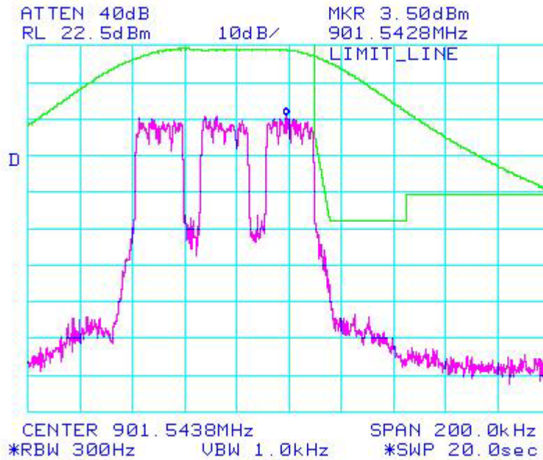
Figure 6b.2.4.3. WiDEN 75 NBPCS Band, Quad- 64 QAM; Occupied Bandwidth
