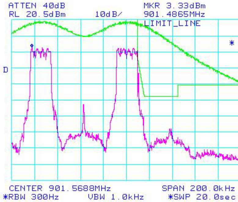
Figure 6b.2.6.1. WiDEN50 Split 900 MHz Band, QPSK; Occupied Bandwidth
