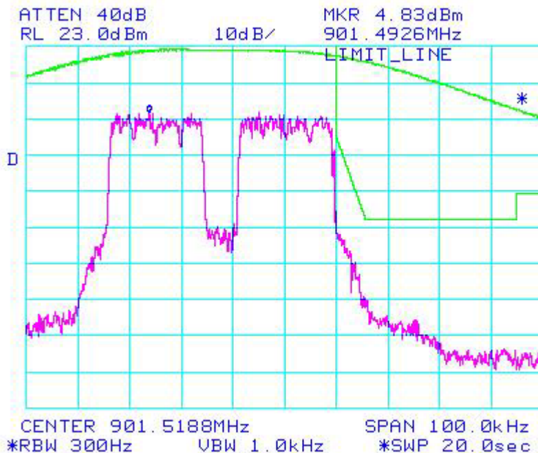
Figure 6b.2.3.3. WiDEN 50 NBPCS Band, Quad- 64 QAM; Occupied Bandwidth
