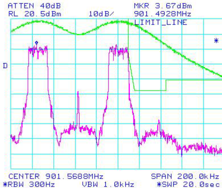
Figure 6b.2.6.2. WiDEN50 Split NBPCS Band, Quad-16 QAM; Occupied Bandwidth
