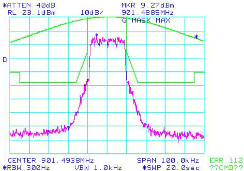
Figure 6b.2.2.2. WiDEN 25 NBPCS Band, Quad-16 QAM; Occupied Bandwidth
