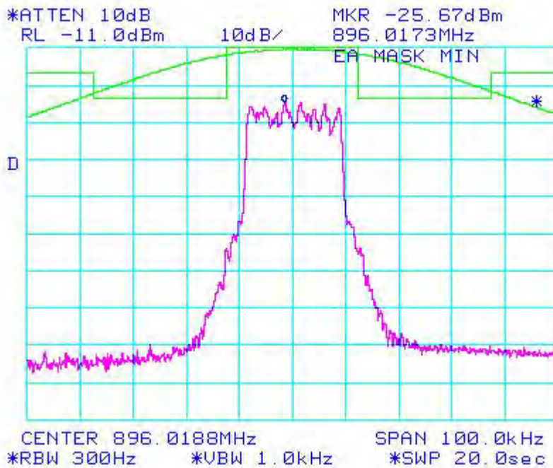
Figure 6a-2.8.12. WiDEN25 900 MHz Band, QAM64, Minimum Power, EA Emission Mask
