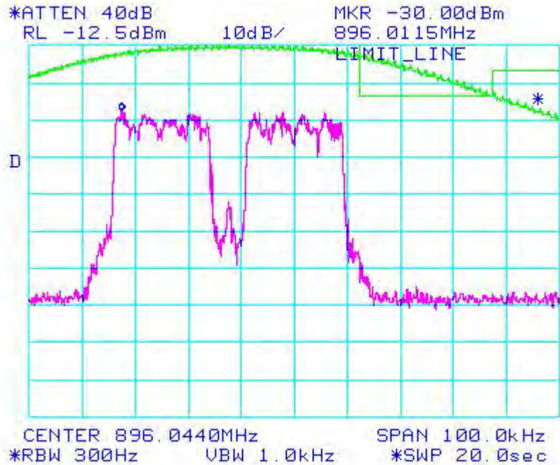
Figure 6a-2.9.2. WiDEN50 900 MHz Band, Continuous Quad-QPSK, Minimum Power, EA Emission Mask
