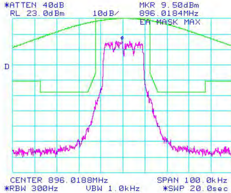
Figure 6a-2.8.11. WiDEN25 900 MHz Band, QAM64, Maximum Power, EA Emission Mask
