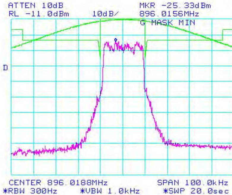
Figure 6a-2.8.2. WiDEN25 900 MHz Band, Quad-QPSK, Minimum Power, Emission Mask G
