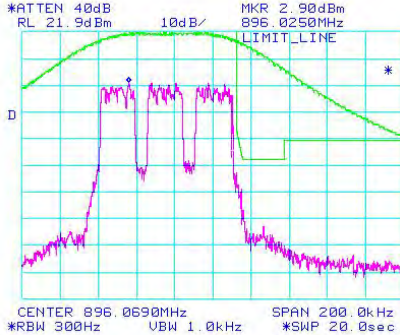
Figure 6a-2.10.1. WiDEN75 900 MHz Band, Quad-QPSK, Maximum Power, EA Emission Mask
