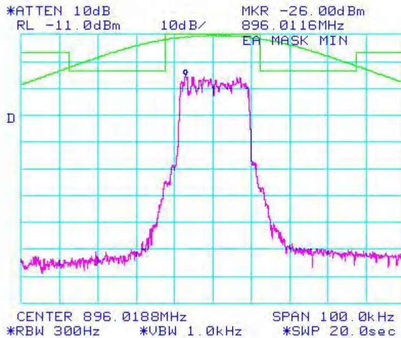
Figure 6a-2.8.8. WiDEN25 900 MHz Band, QAM16, Minimum Power, EA Emission Mask
