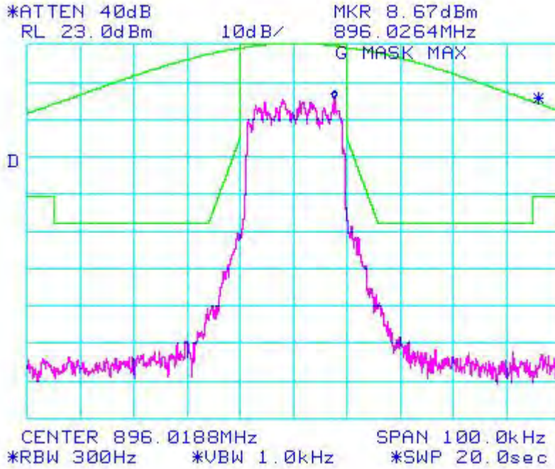
Figure 6a-2.8.1. WiDEN25 900 MHz Band, Quad-QPSK, Maximum Power, Emission Mask G
