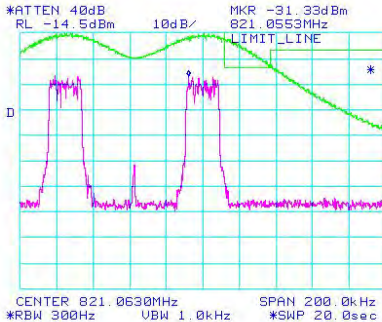
Figure 6a-2.7.4. WiDEN50 Split 800 MHz Band, QAM16, Minimum Power, EA Emission Mask
