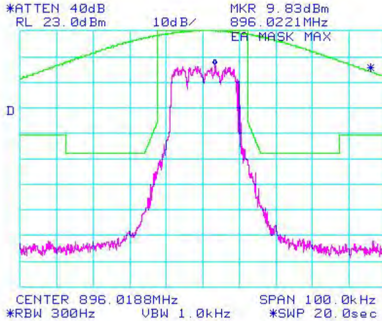
Figure 6a-2.8.7. WiDEN25 900 MHz Band, QAM16, Maximum Power, EA Emission Mask
