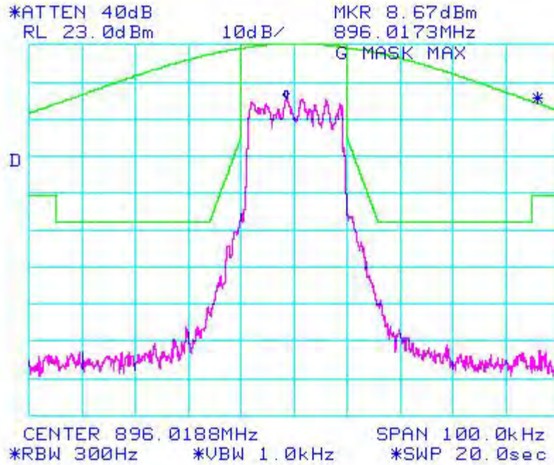
Figure 6a-2.8.9. WiDEN25 900 MHz Band, QAM64, Maximum Power, Emission Mask G
