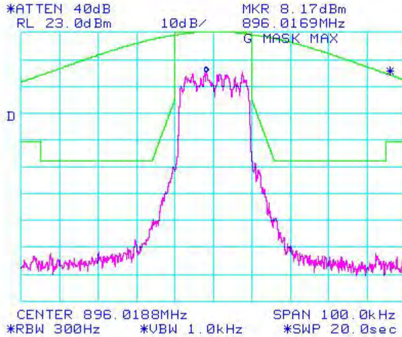
Figure 6a-2.8.5. WiDEN25 900 MHz Band, QAM16, Maximum Power, Emission Mask G
