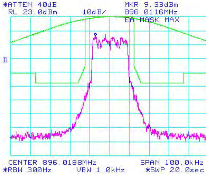
Figure 6a-2.8.3. WiDEN25 900 MHz Band, Quad-QPSK, Maximum Power, EA Emission Mask
