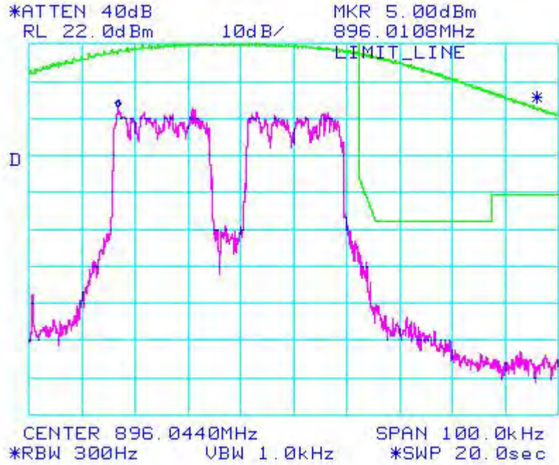
Figure 6a-2.9.1. WiDEN50 900 MHz Band, Continuous Quad-QPSK, Maximum Power, EA Emission Mask
