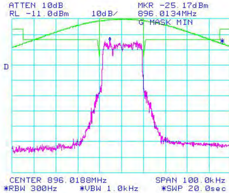
Figure 6a-2.8.6. WiDEN25 900 MHz Band, QAM16, Minimum Power, Emission Mask G
