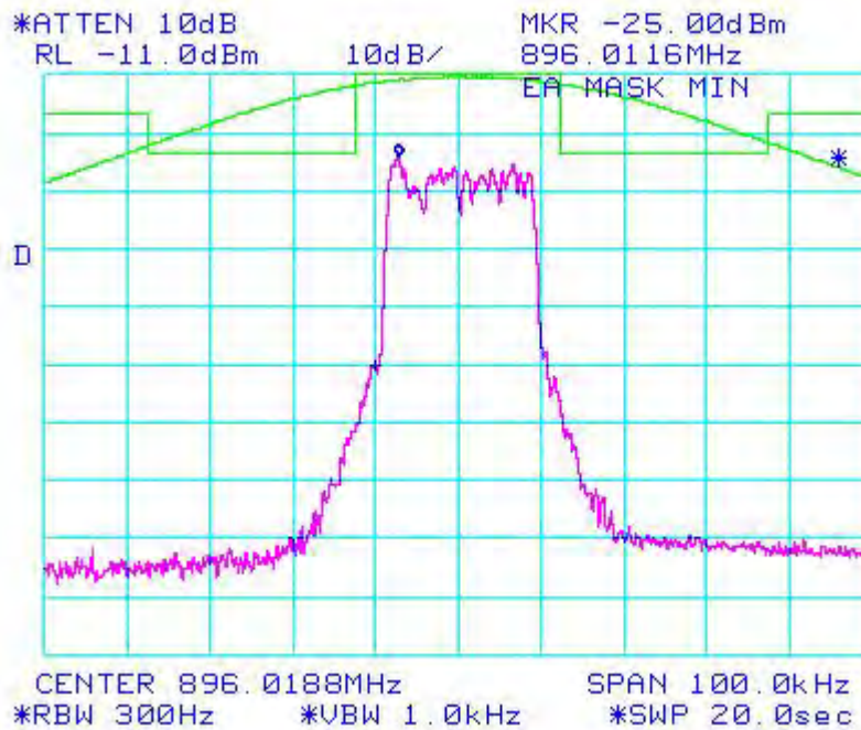
Figure 6a-2.8.4. WiDEN25 900 MHz Band, Quad-QPSK, Minimum Power, EA Emission Mask
