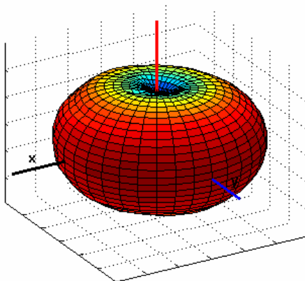
Figure 6b.6.1: i290 Antenna Pattern at NBPCS frequency band.
