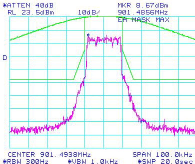
Figure 6b.2.1.3. iDEN NBPCS Band, Quad- 64QAM; Occupied Bandwidth
