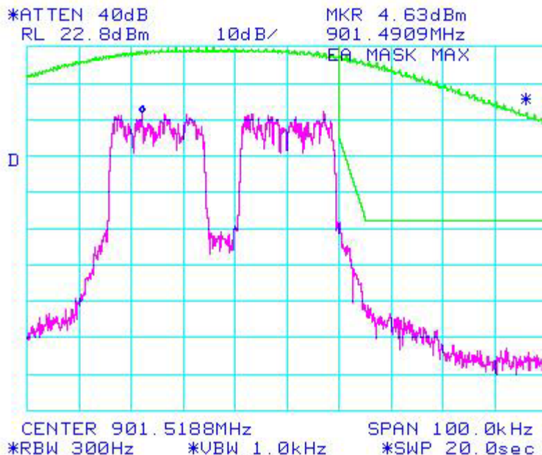
Figure 6b.2.1.7. WiDEN 50 NBPCS Band, QPSK; Occupied Bandwidth
