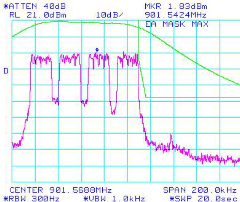
Figure 6b.2.1.14. WiDEN 100 NBPCS Band, Quad- 16 QAM; Occupied Bandwidth
