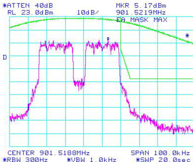
Figure 6b.2.1.8. WiDEN 50 NBPCS Band, Quad- 16 QAM; Occupied Bandwidth
