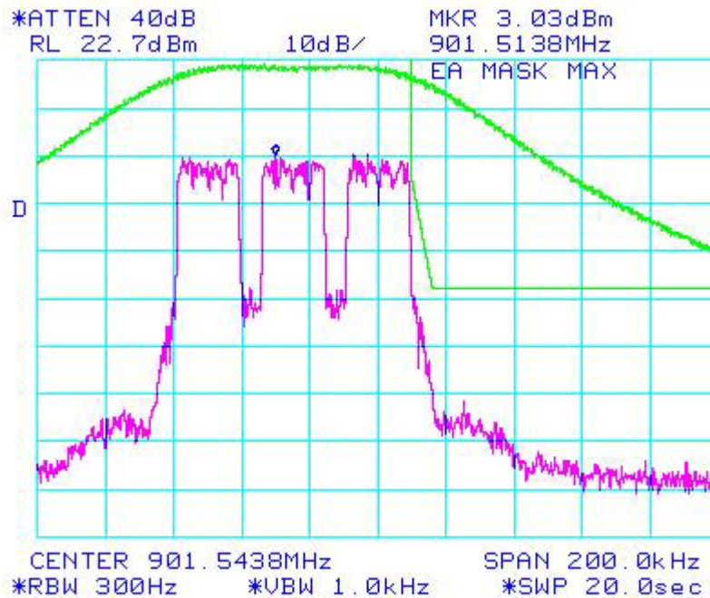
Figure 6b.2.1.12. WiDEN 75 NBPCS Band, Quad- 64 QAM; Occupied Bandwidth
