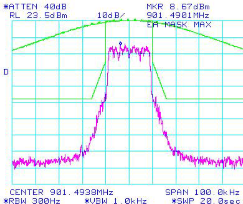
Figure 6b.2.1.5. WiDEN 25 NBPCS Band, Quad- 16 QAM; Occupied Bandwidth
