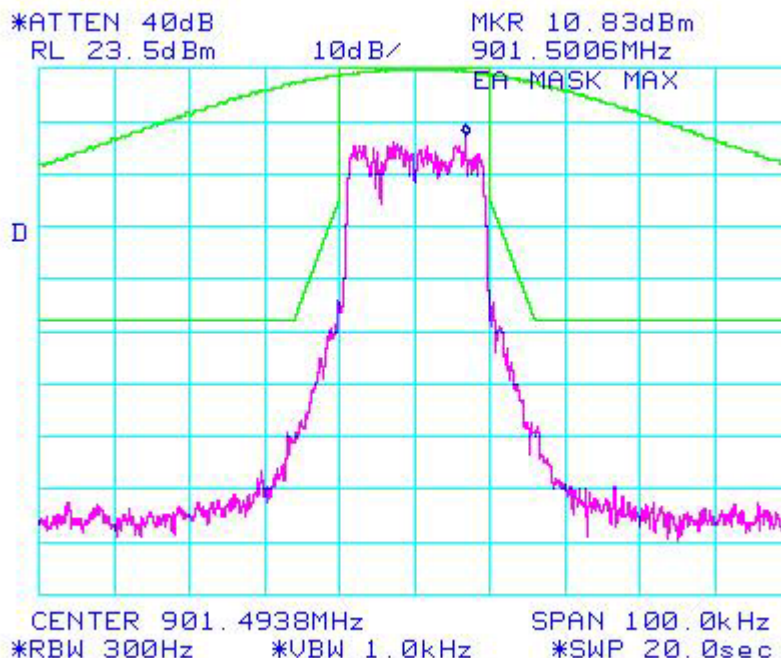
Figure 6b.2.1.4. WiDEN 25 900 MHz Band, QPSK, Occupied Bandwidth
