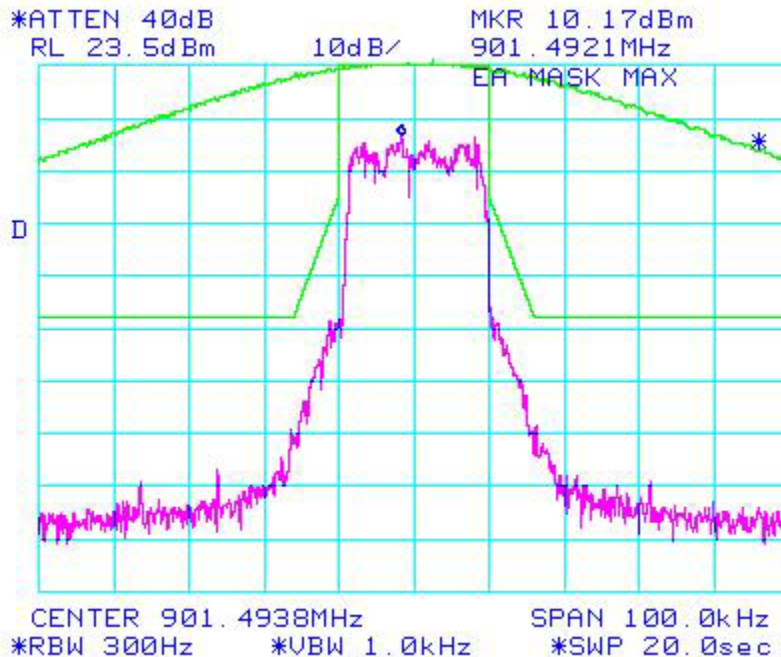
Figure 6b.2.1.1 iDEN NBPCS Band, QPSK; Occupied Bandwidth.
