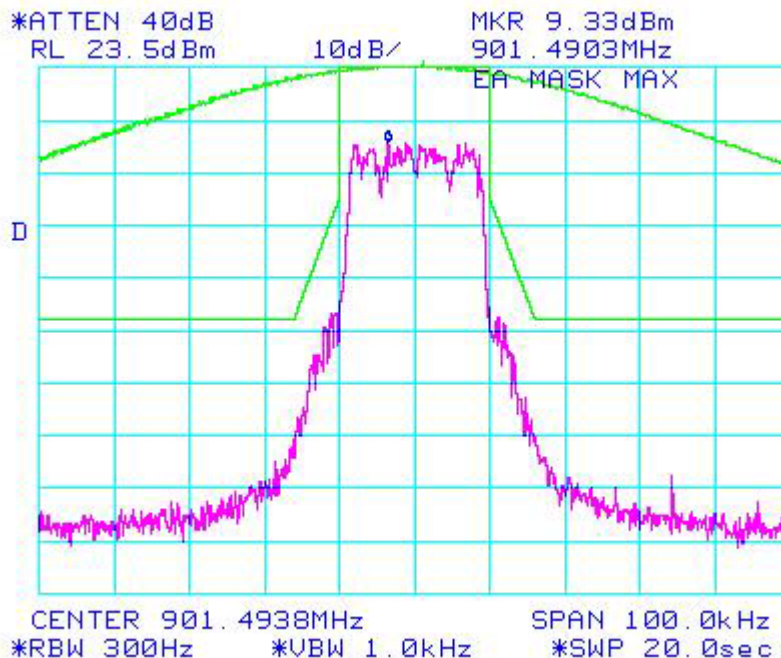
Figure 6b.2.1.2. iDEN NBPCS Band, Quad-16QAM; Occupied Bandwidth
