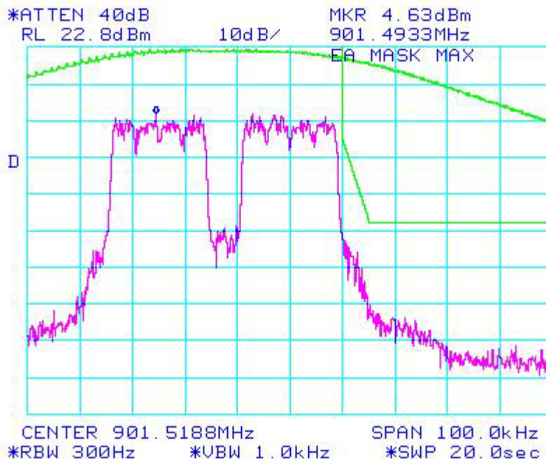
Figure 6b.2.1.9. WiDEN 50 NBPCS Band, Quad- 64 QAM; Occupied Bandwidth
