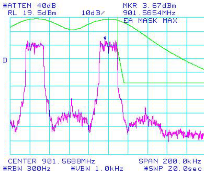
Figure 6b.2.1.17. WiDEN 50_Split NBPCS Band, Quad- 16 QAM; Occupied Bandwidth
