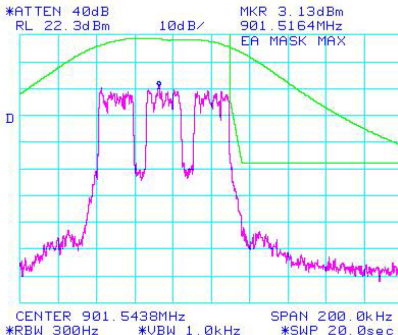
Figure 6b.2.1.10. WiDEN 75 NBPCS MHz Band, QPSK; Occupied Bandwidth
