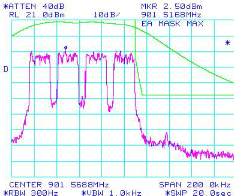
Figure 6b.2.1.13. WiDEN 100 NBPCS Band, QPSK; Occupied Bandwidth
