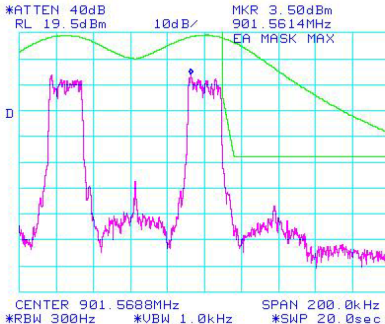
Figure 6b.2.1.16. WiDEN 50_Split 900 MHz Band, QPSK; Occupied Bandwidth
