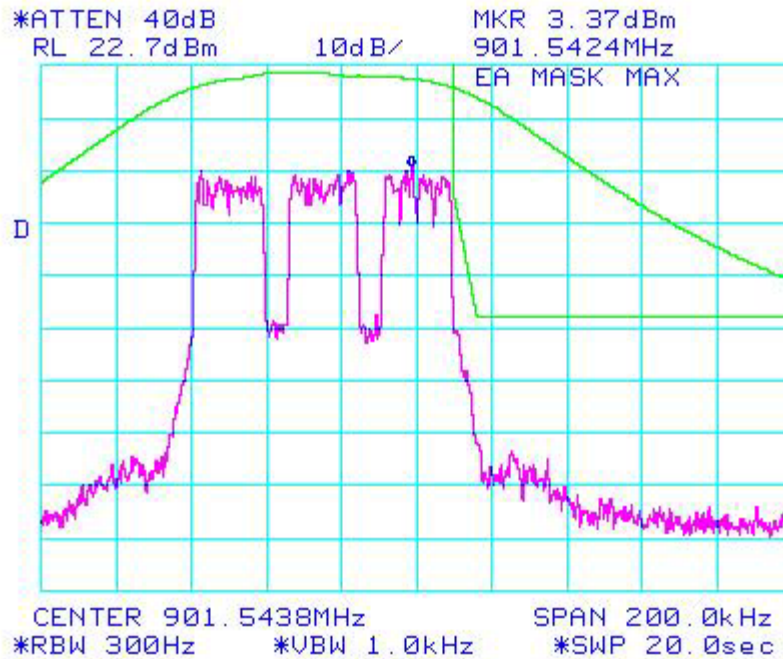
Figure 6b.2.1.11. WiDEN 75 NBPCS Band, Quad- 16 QAM; Occupied Bandwidth
