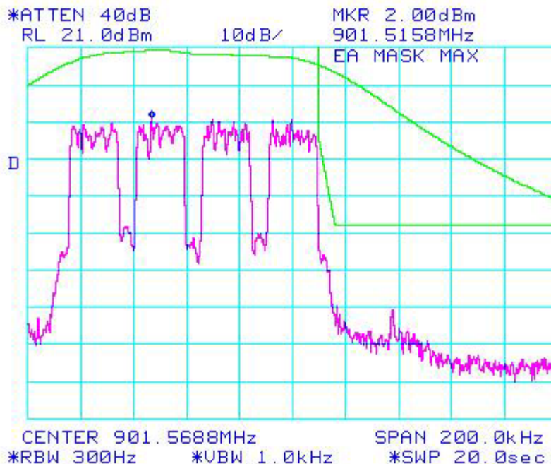
Figure 6b.2.1.15. WiDEN 100 NBPCS Band, Quad-64 QAM; Occupied Bandwidth
