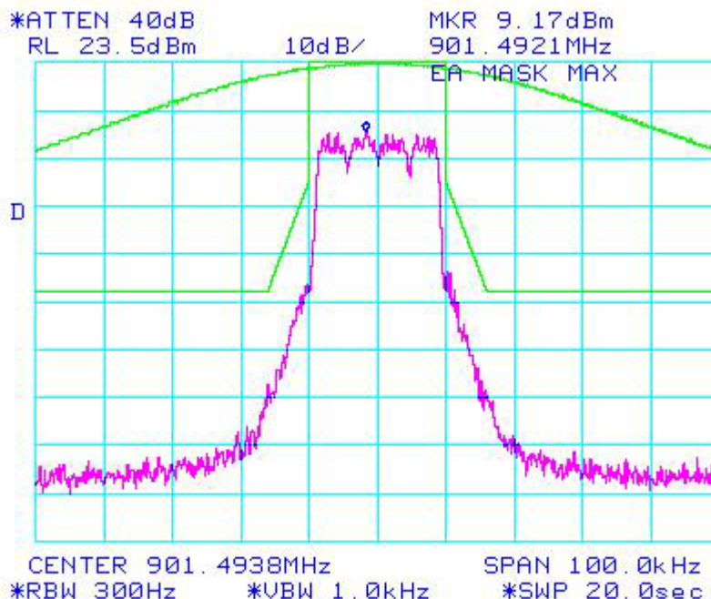
Figure 6b.2.1.6. WiDEN 25 NBPCS Band, Quad- 64 QAM; Occupied Bandwidth
