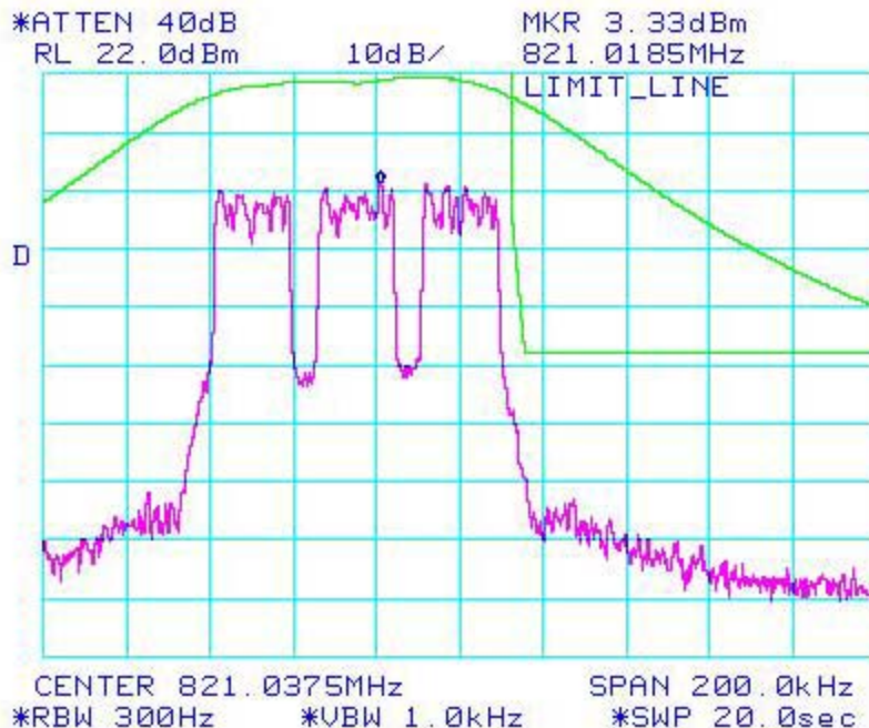
Figure 6a-2.5.1. WiDEN75 800 MHz Band, Quad-QPSK, Maximum Power, EA Emission Mask
