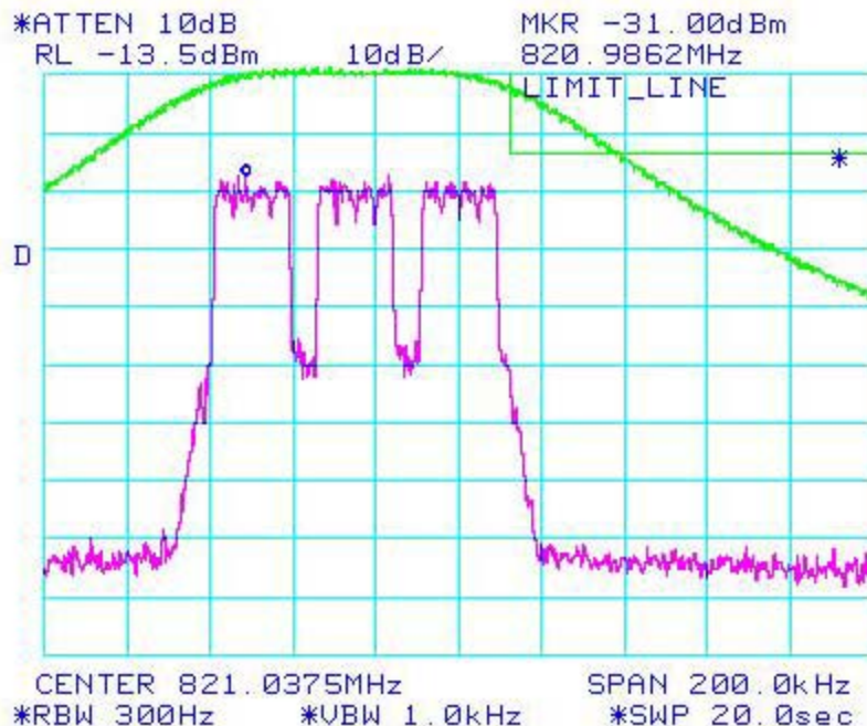
Figure 6a-2.5.6. WiDEN75 800 MHz Band, QAM64, Minimum Power, EA Emission Mask
