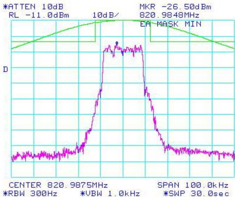
Figure 6a-2.3.12. WiDEN25 800 MHz Band, QAM64, Minimum Power, EA Emission Mask
