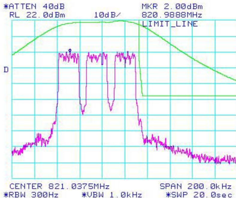
Figure 6a-2.5.5. WiDEN75 800 MHz Band, QAM64, Maximum Power, EA Emission Mask
