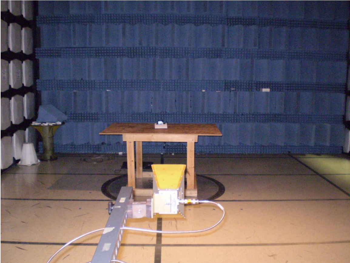
Tx Radiated
