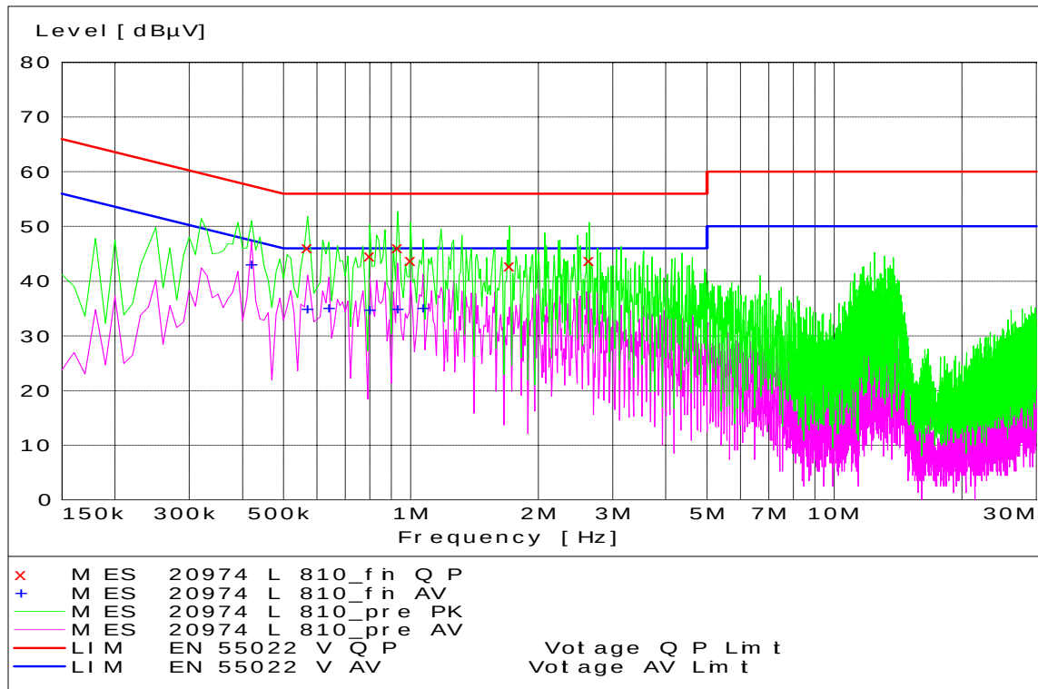
PCS Channel 810 - Tx Mode -Line
