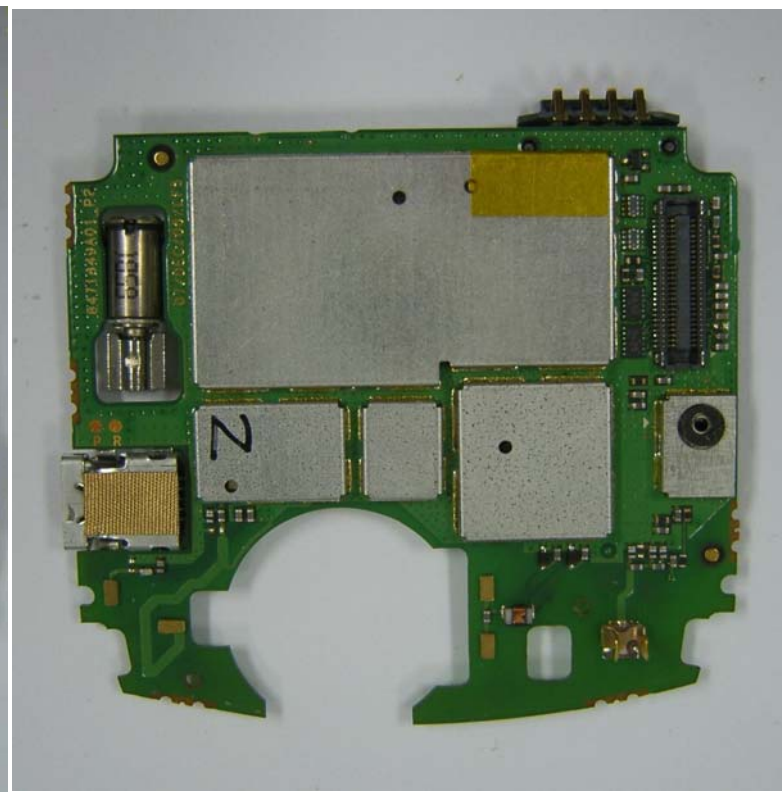
Main Board(Shield on)
