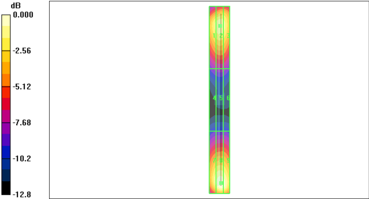
0 dB = 166.1V/m
