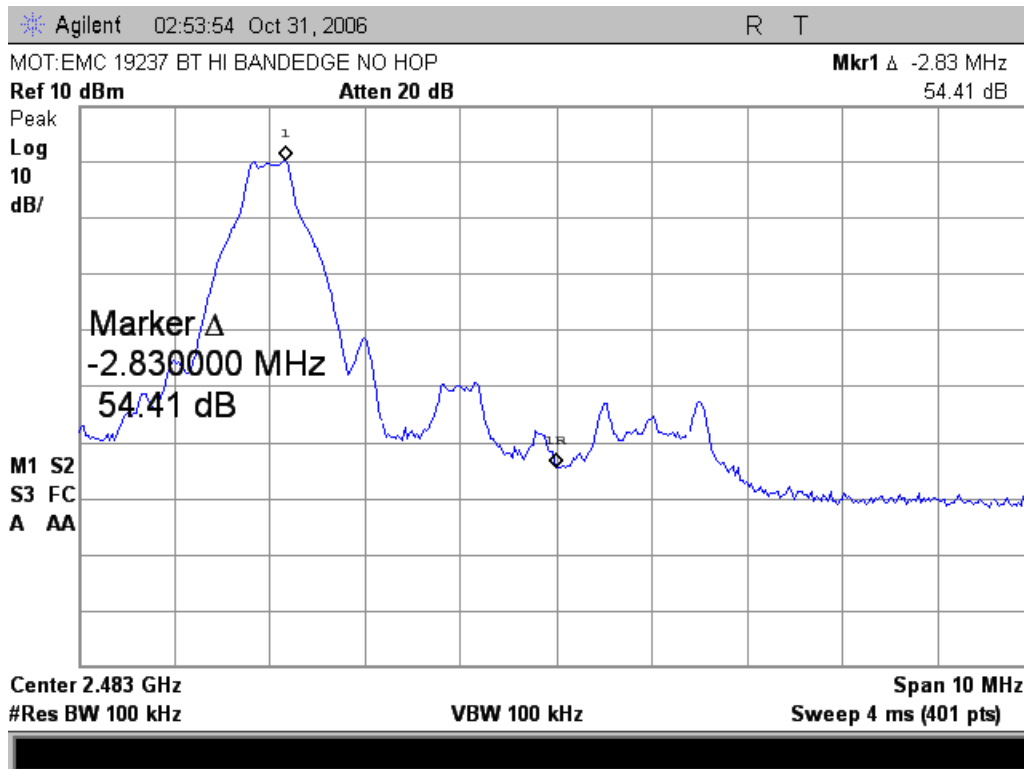
High Band Edge with Hopping Disabled
