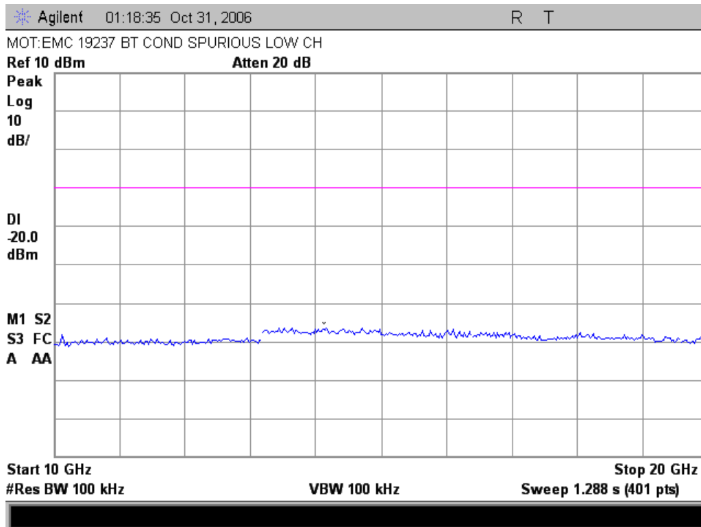
Conducted Spurious Emissions 10-20GHz (Low Channel Enabled)
