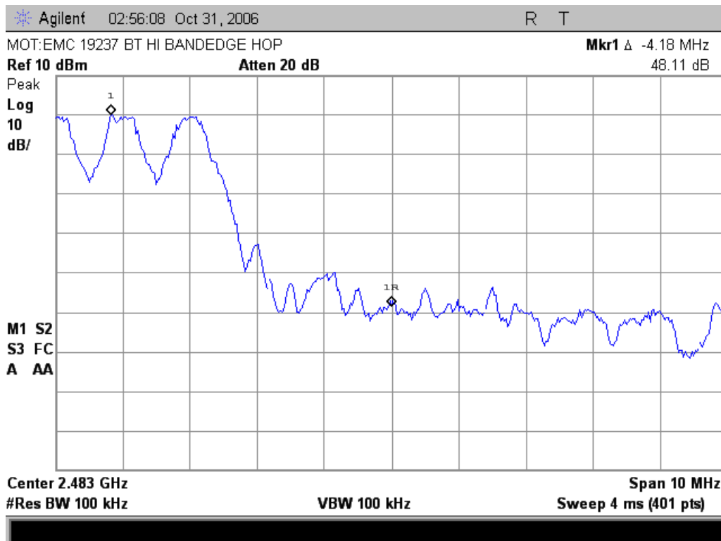
High Band Edge with Hopping Enabled
