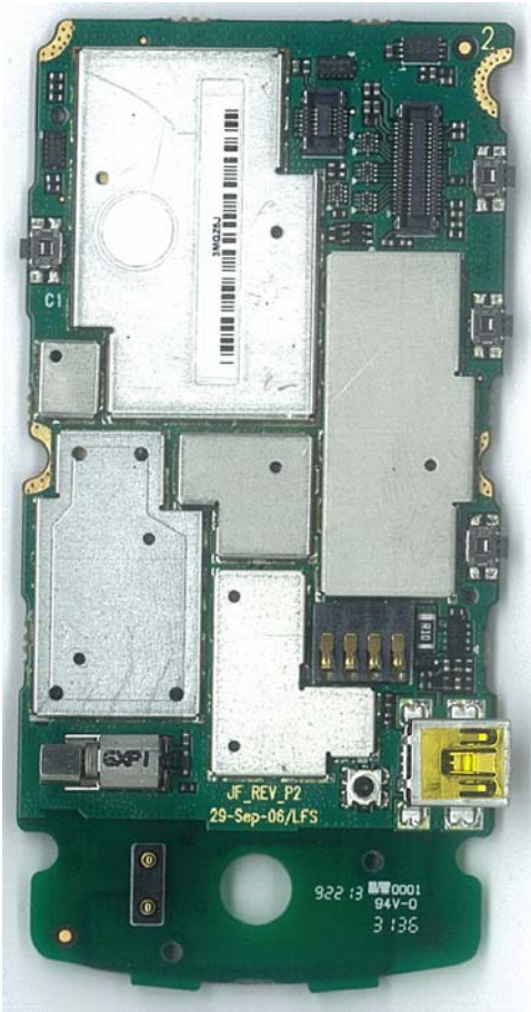
Main PCB Bottom View
