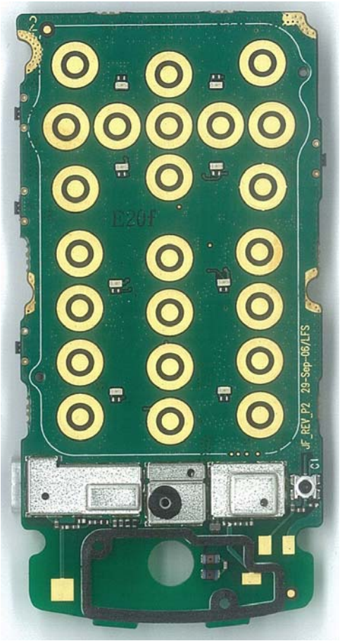
Main PCB Key-Side View without Key-Dome
