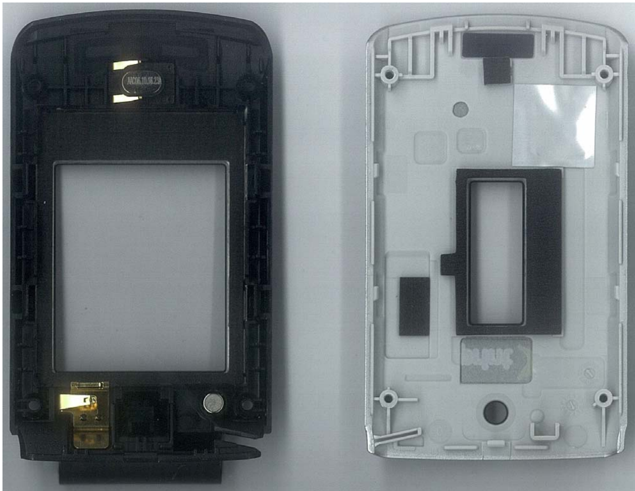
Inside Front housing of Flip Board
