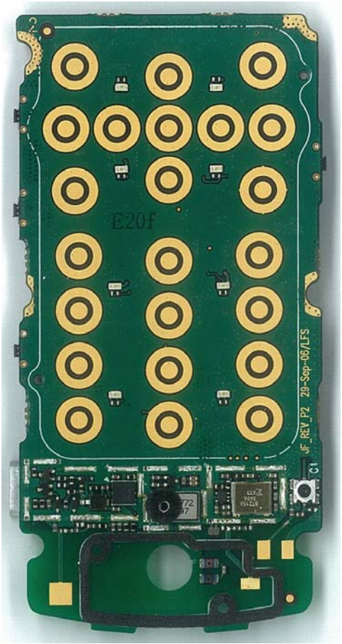
Main PCB Key-Side View without Shields
