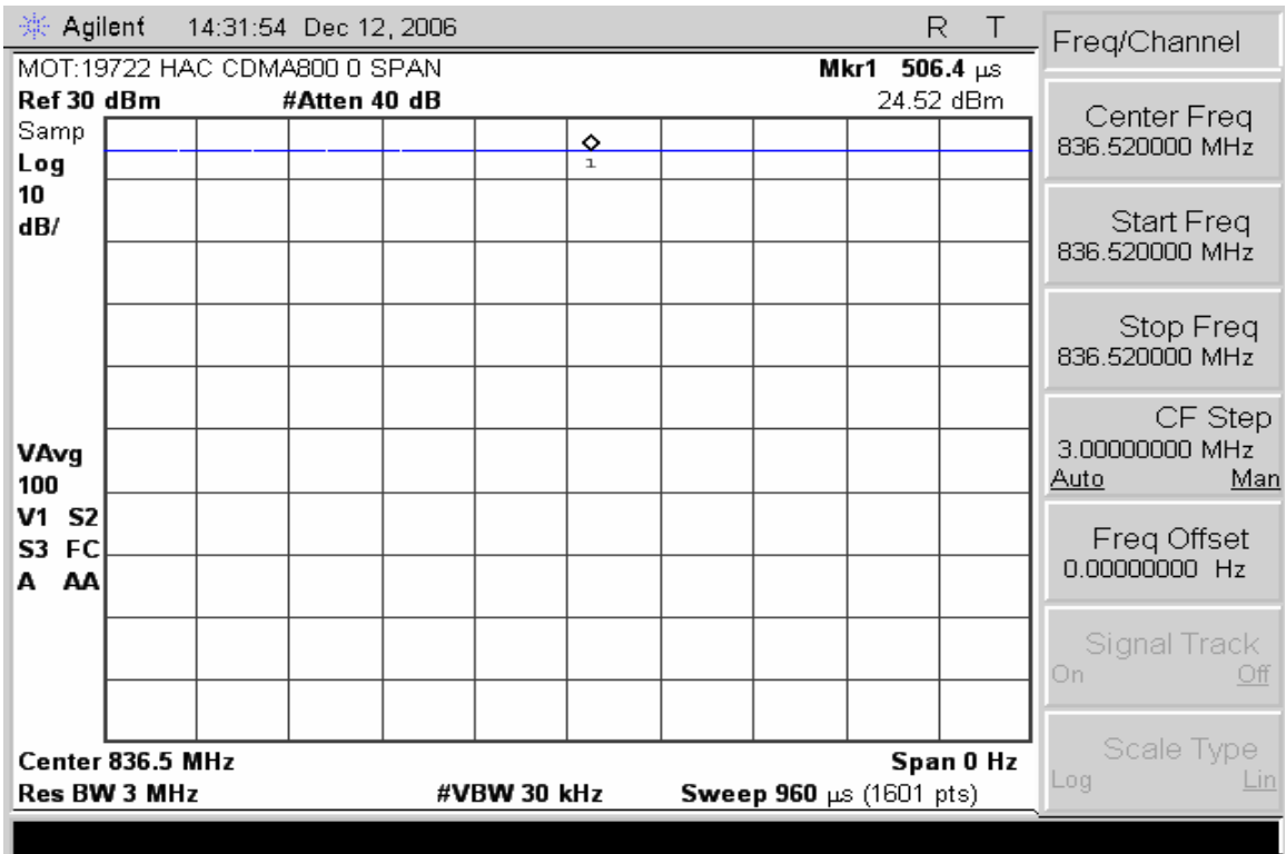
836.52 MHz (0 span)
