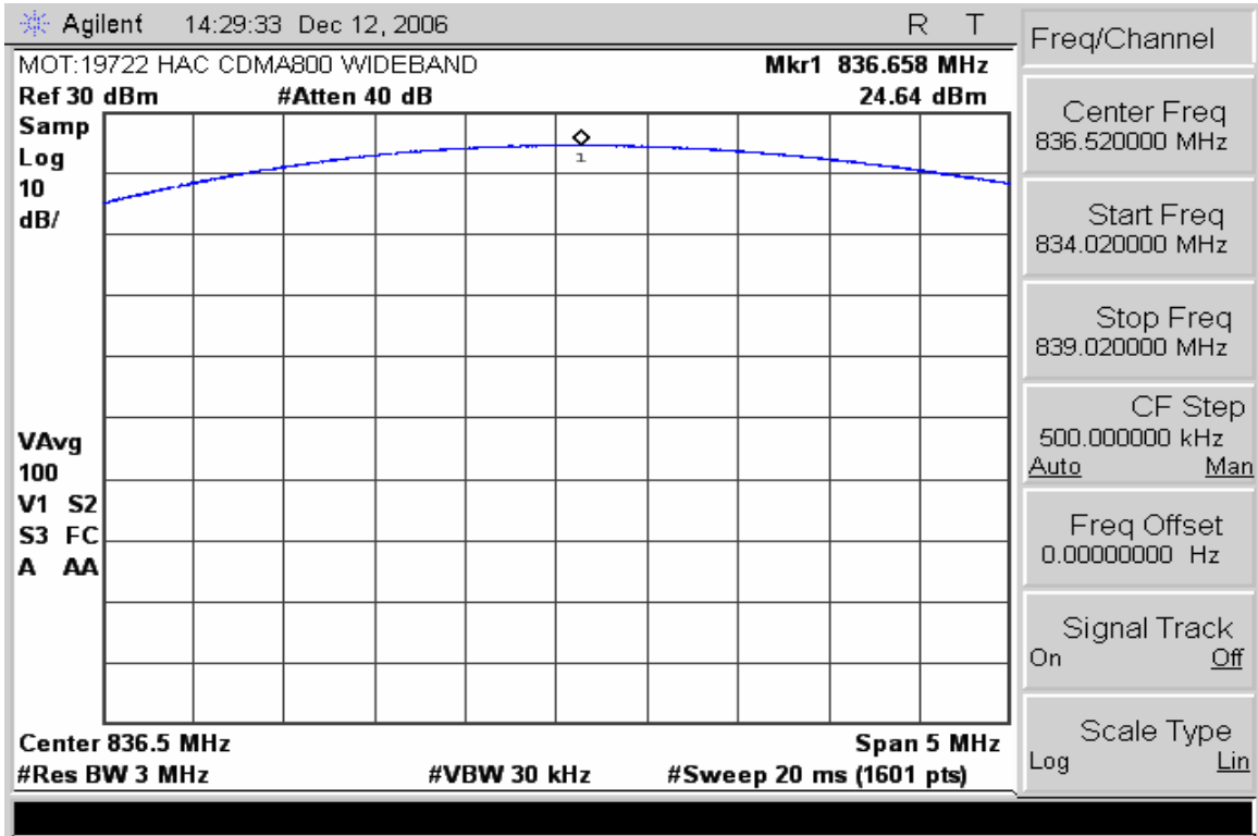
836.52 MHz (wideband)
