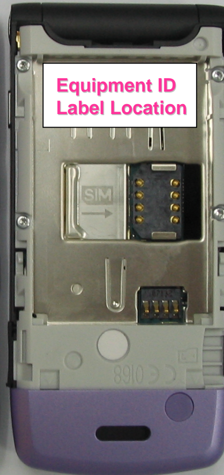
Rear View with Battery Door removed, showing ID Label
