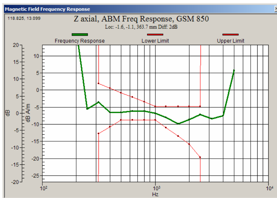
Graph 2: GSM 850 Frequency Response
