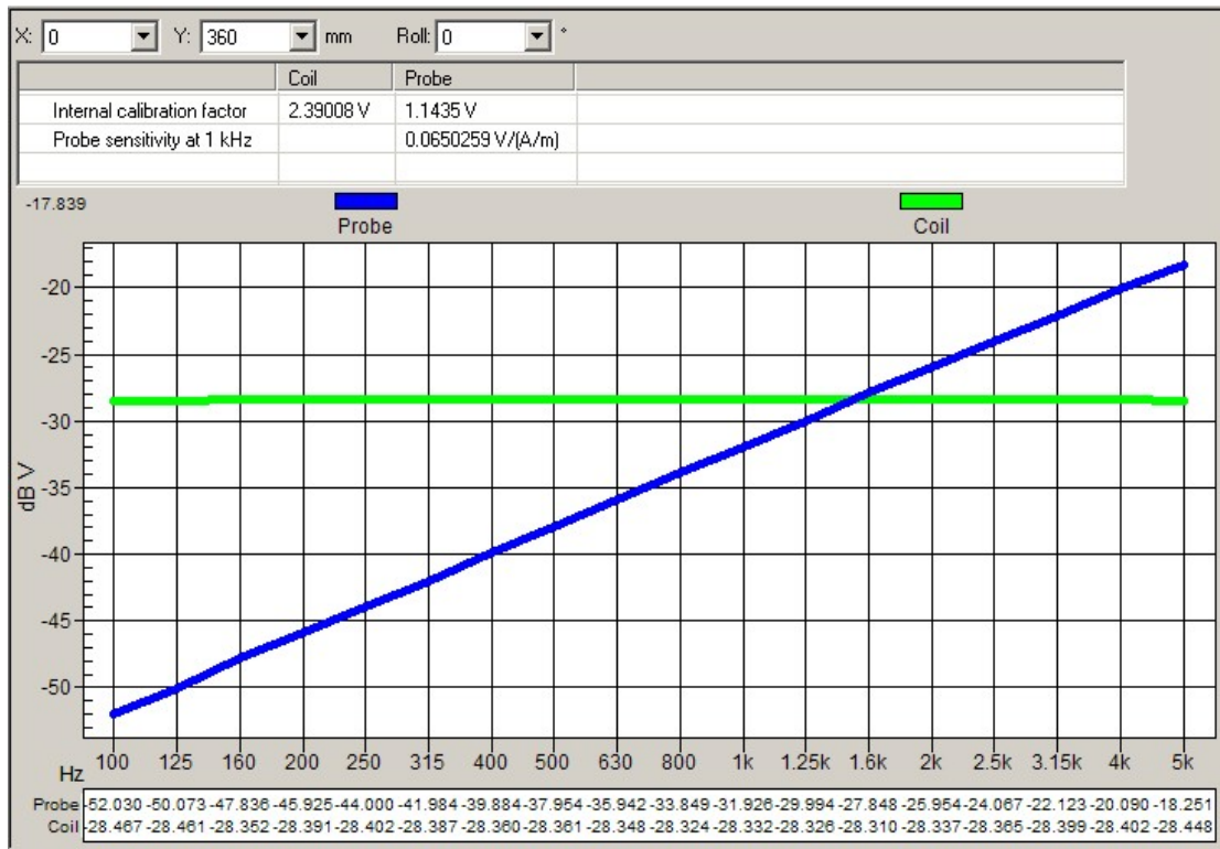
Graph 1: Frequency Response measured in AMCC
