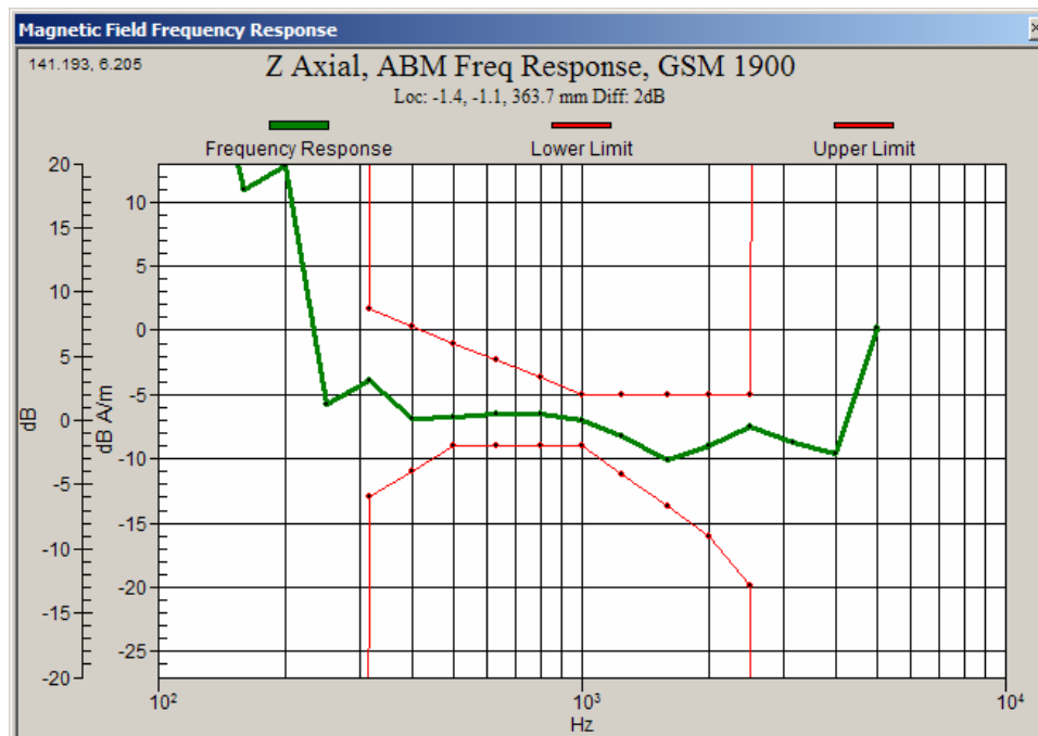
Graph 3: GSM 1900 Frequency Response
