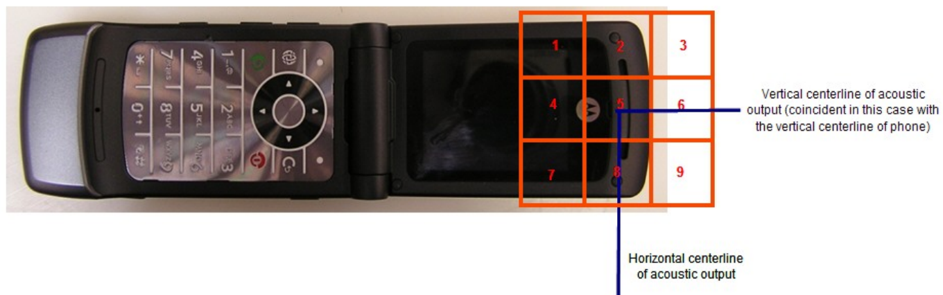
Figure A5-2. Phone Open - Orientation of Wireless Device and Measurement Plane
