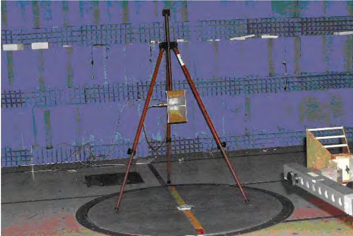
EMC Report #19754-1, Antenna - Substitution
