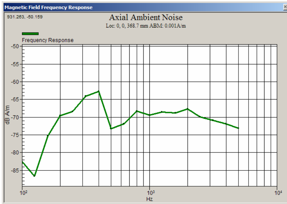
Graph A2-1. Axial Orientation Ambient Noise Spectrum Plot
