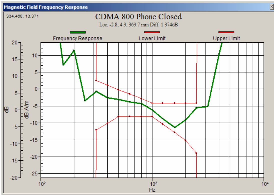
Graph 2: CDMA 800 Frequency Response (Slide Closed)
