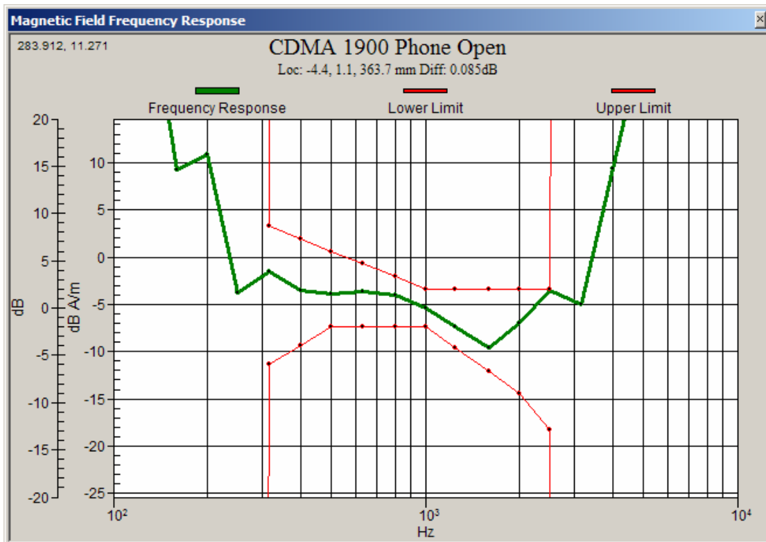
Graph 5: CDMA 1900 Frequency Response (Slide Open)
