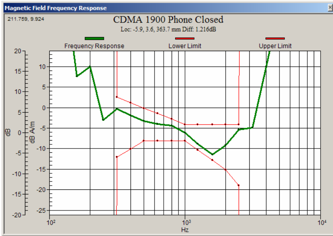
Graph 4: CDMA 1900 Frequency Response (Slide Closed)
