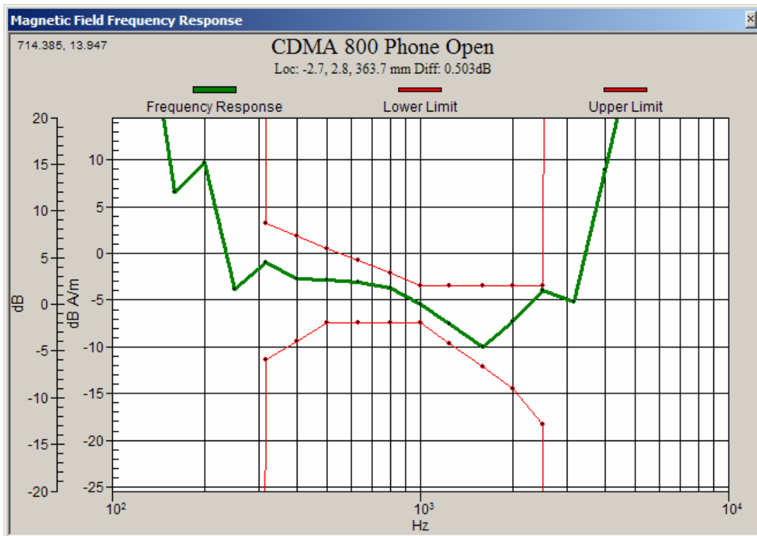
Graph 3: CDMA 800 Frequency Response (Slide Open)
