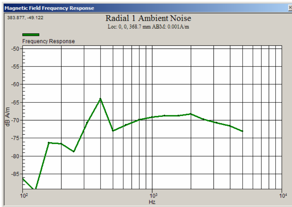
Graph A2-2. Radial 1 Orientation Ambient Noise Spectrum Plot
