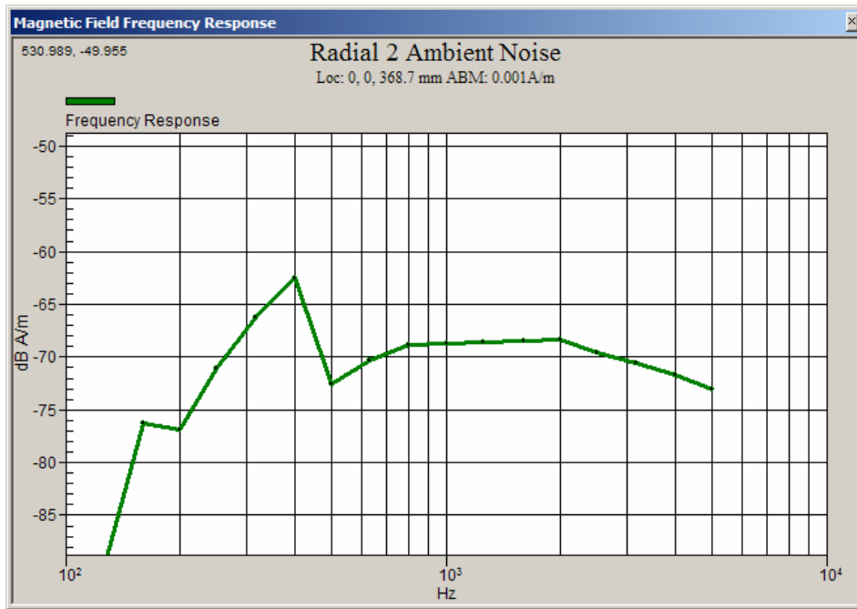
Graph A2-3. Radial 2 Orientation Ambient Noise Spectrum Plot
