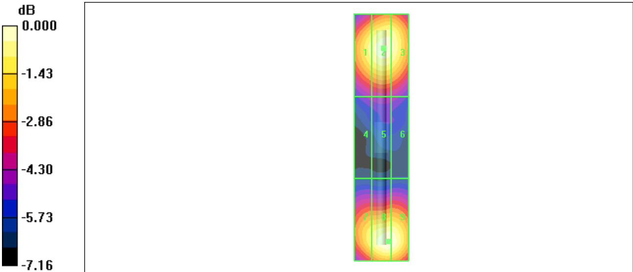
0 dB = 131.7V/m
