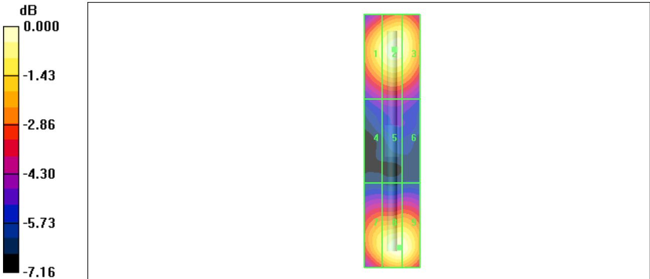
0 dB = 131.7V/m
