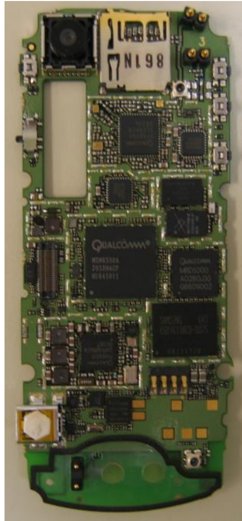
Main Board Bottom Without Shields
