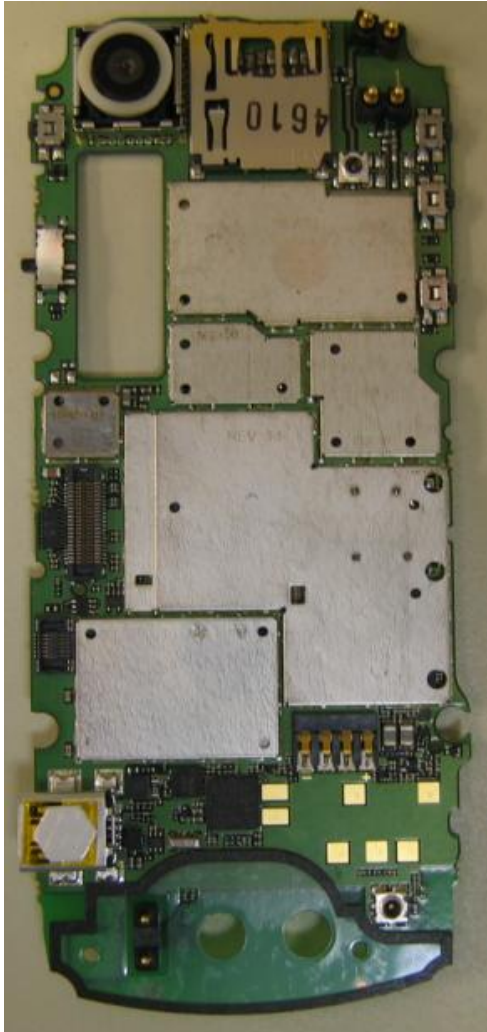
Main Board Bottom With Shields
