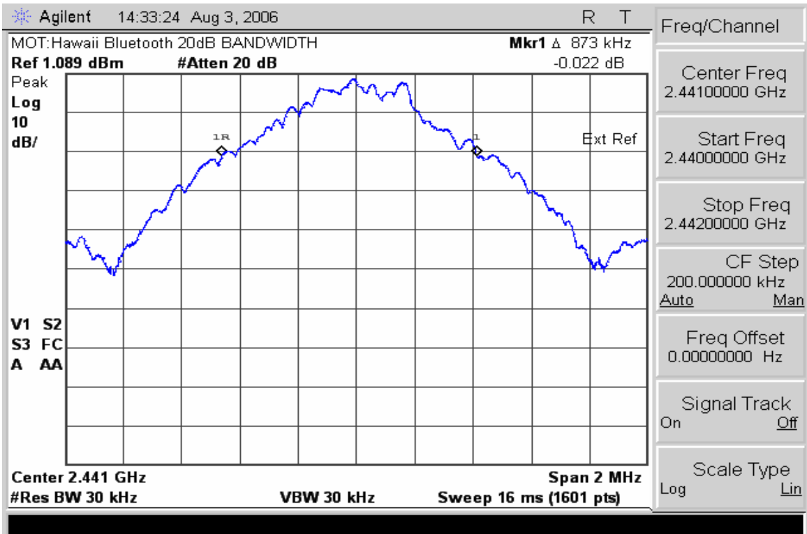
20dB Bandwidth
