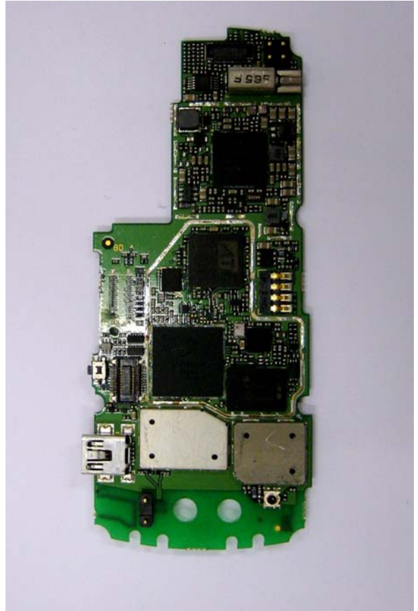
Main Board Bottom Without Shields
