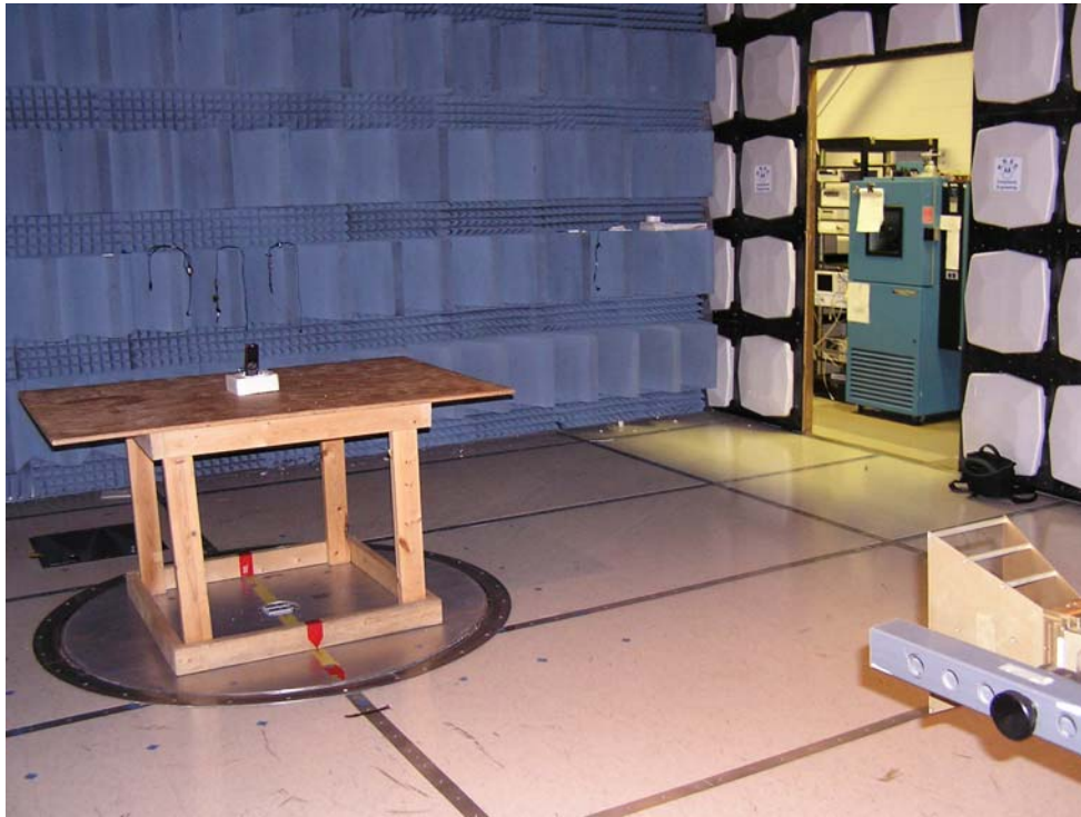
A.1 Radiated Emissions Measurement
