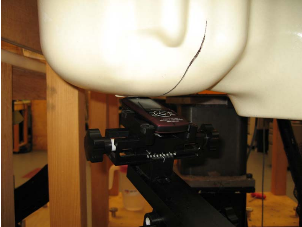
Figure 9 – Transceiver against head, 15° Tilt position, Slider Down
