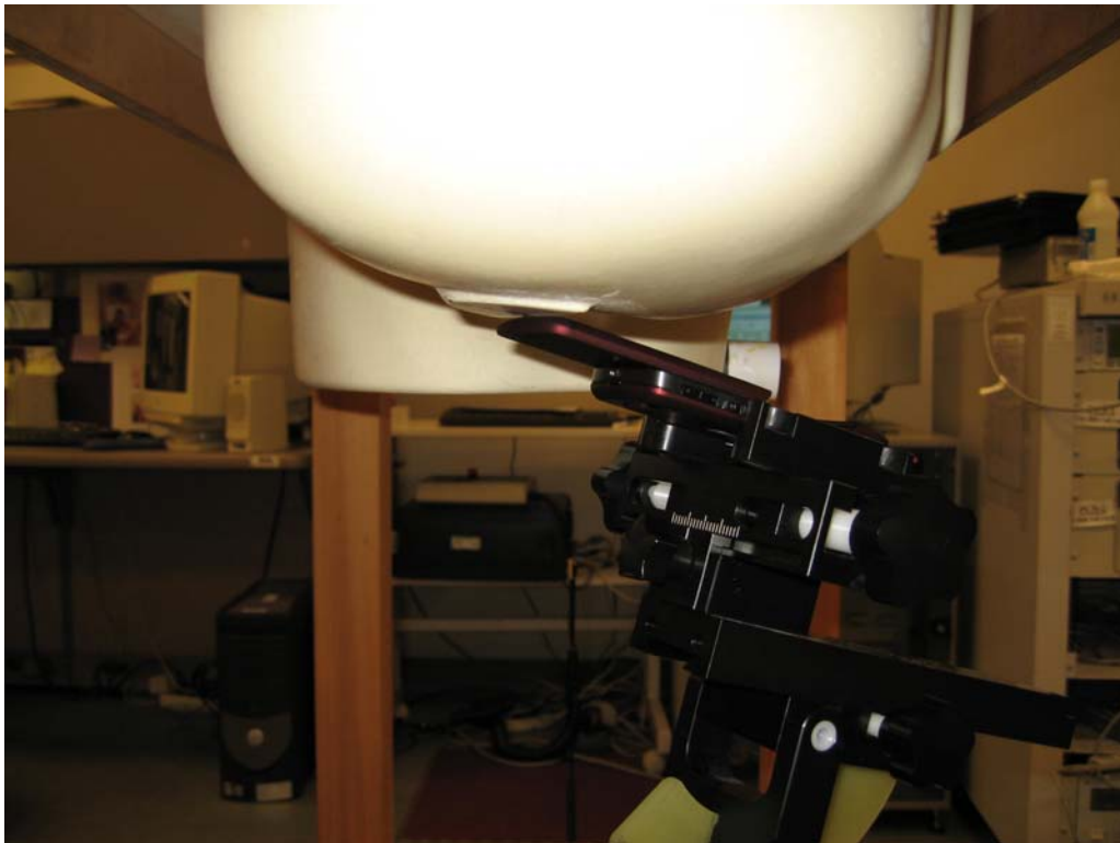
Figure 8 – Transceiver against head, 15° Tilt position, Slider Up
