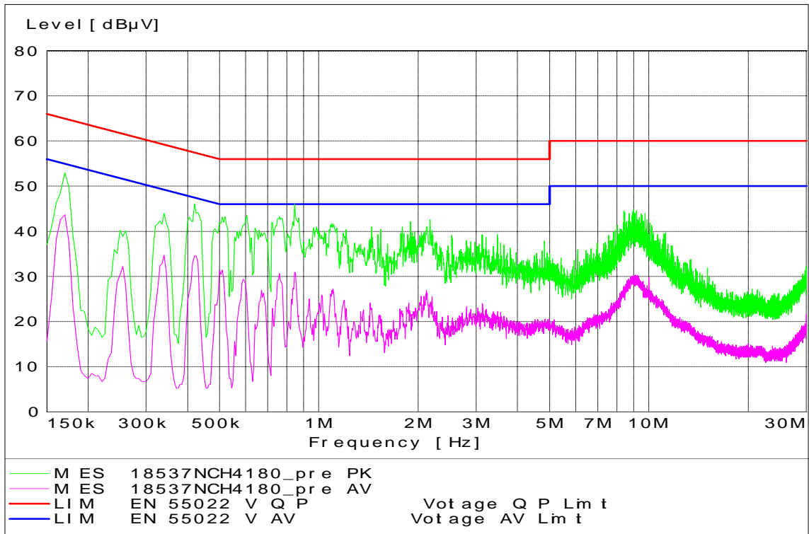
WCDMA850 Channel 4180 - Tx Mode - Neutral Coupling
