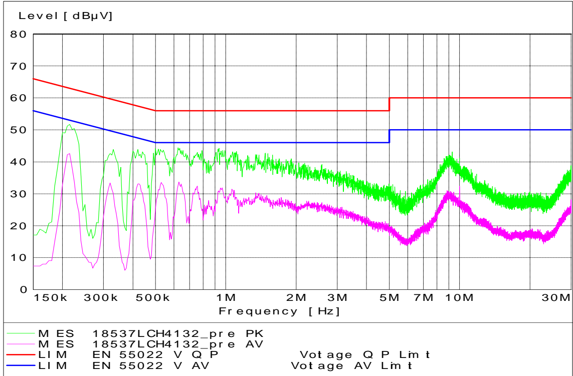
WCDMA850 Channel 4132 - Tx Mode - Line Coupling
