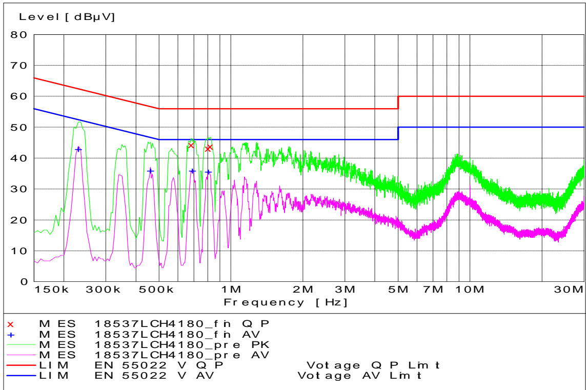
WCDMA850 Channel 4180 - Tx Mode - Line Coupling
