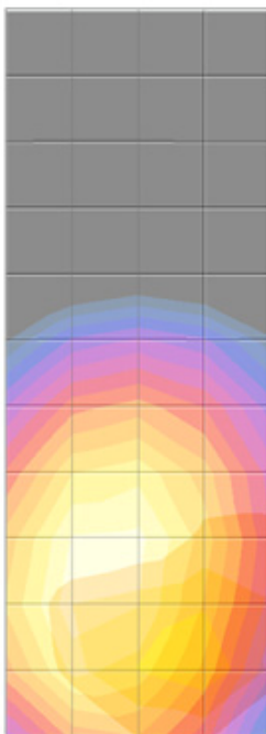
Bluetooth SAR overlaid on GSM850 SAR
