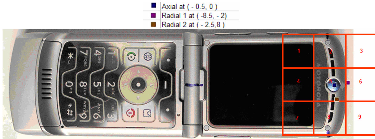
Figure A2-3. Phone Open – 5cm x 5cm grid for Near Field Measurements and T-coil Measured Point locations
