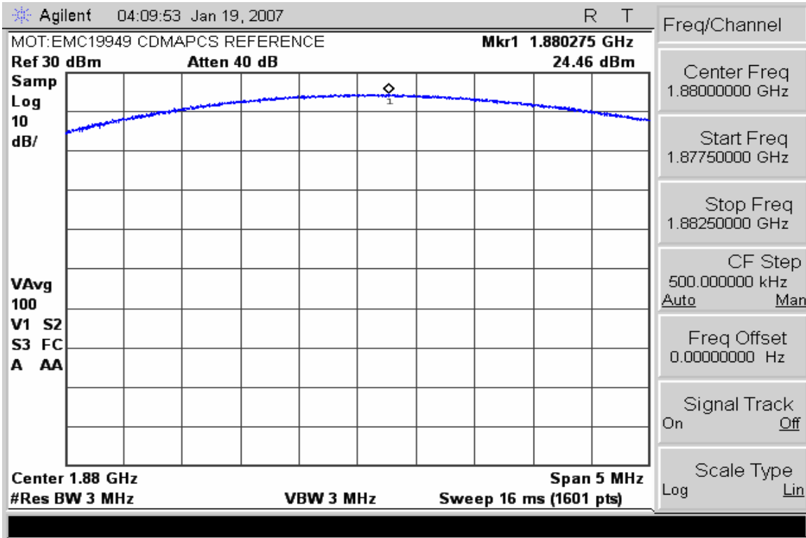
CDMA - PCS Channel 600 Reference Level
