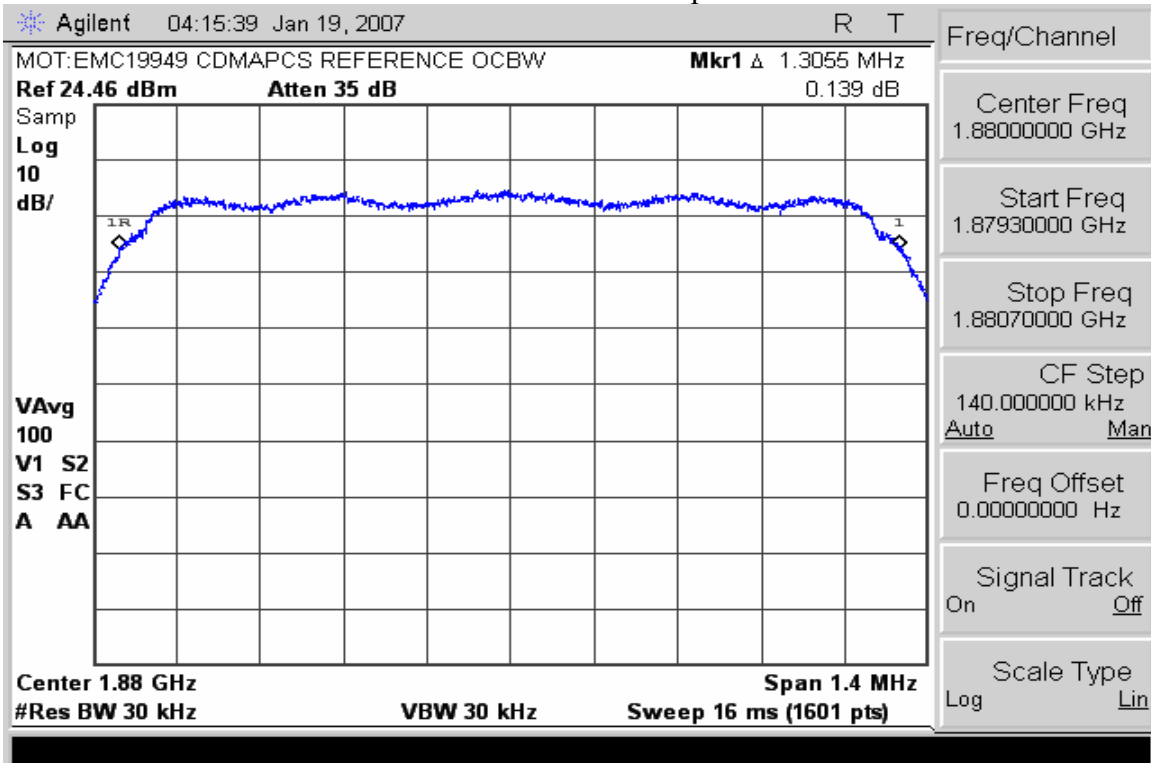
CDMA - PCS Channel 600 Occupied Bandwidth
