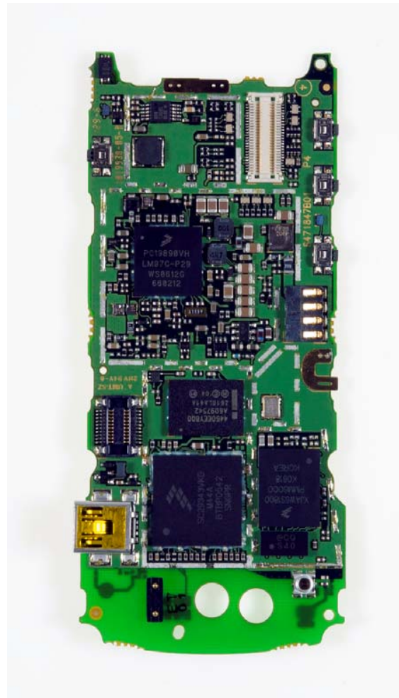
Main Board Bottom Without Shields
