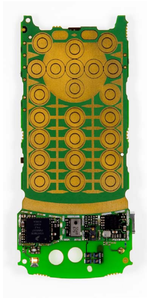
Main Board Top Without Popples or Shields
