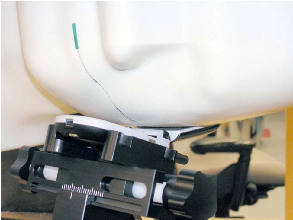
Figure 5. Phone Against the Head with Antenna Retracted (Cheek Touch)
