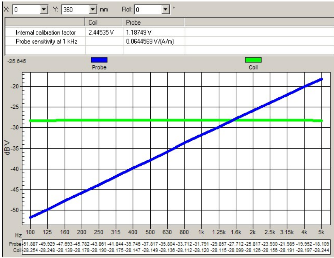
Graph 1: Frequency Response measured in AMCC
