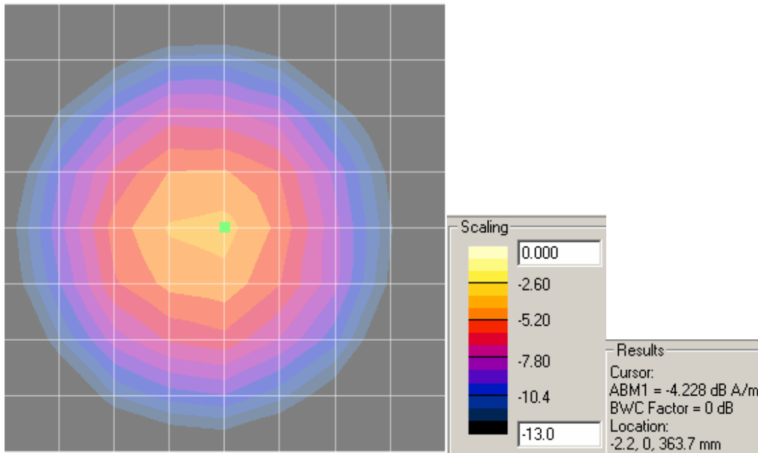
Axial – ABM1
