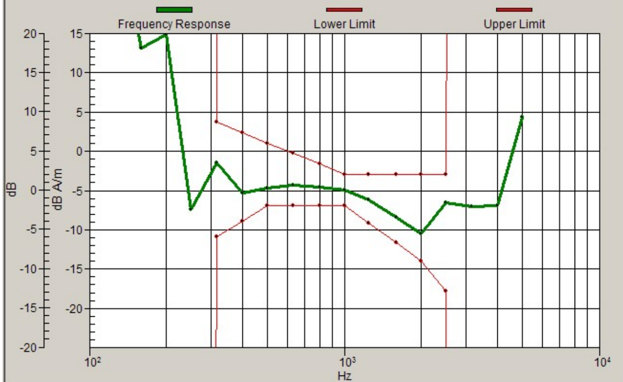
Graph 3: GSM 1900 Frequency Response
