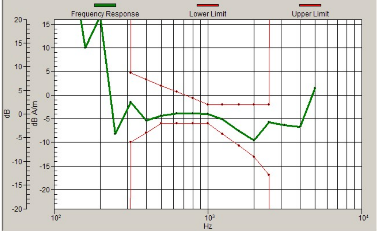
Graph 2: GSM 850 Frequency Response
