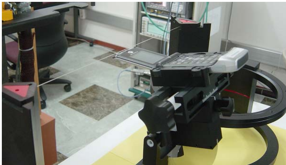
Figure A5-5. Measurement for RF Emissions
