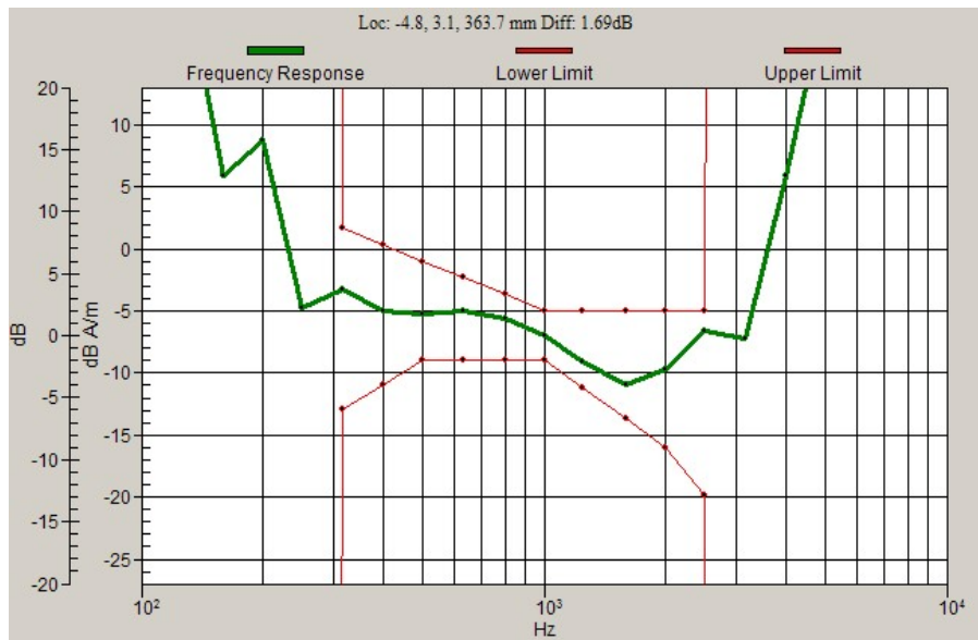
Graph 3: CDMA 800 Frequency Response with Battery 2
