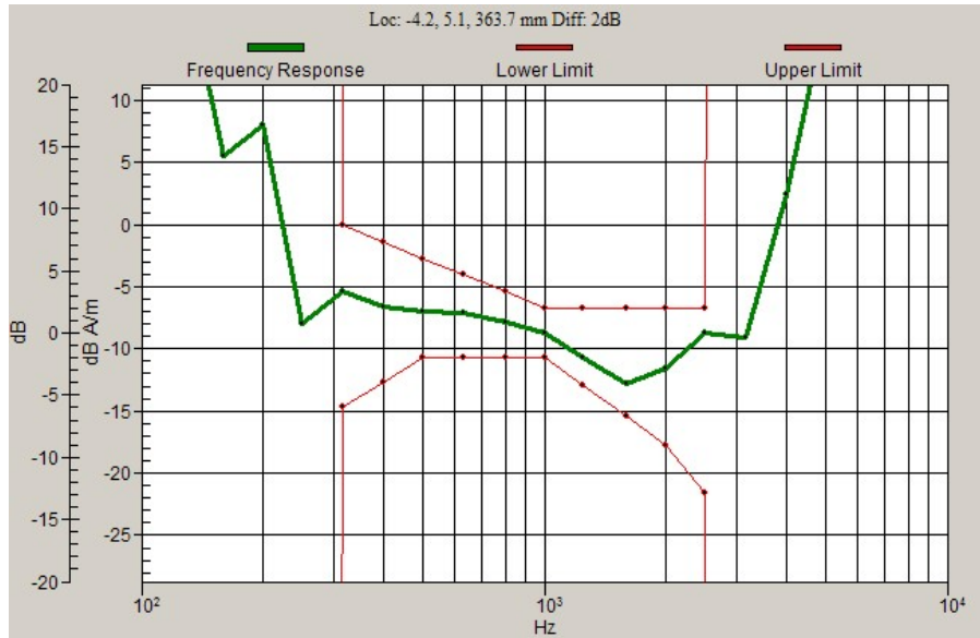
Graph 2: CDMA 800 Frequency Response
