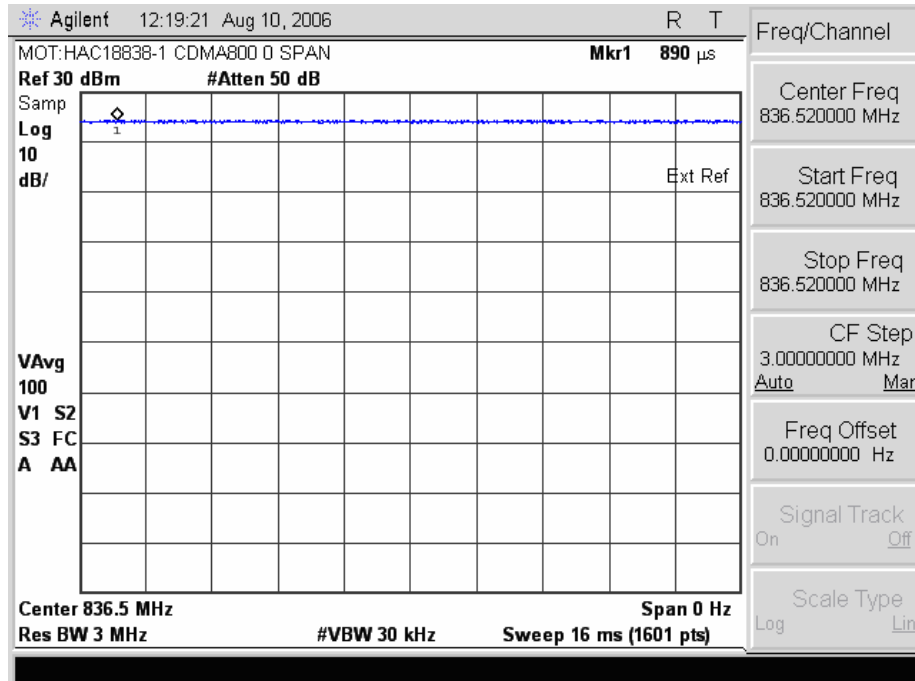
836.52 MHz (0 span)
