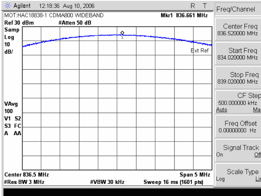
836.52 MHz (wideband)
